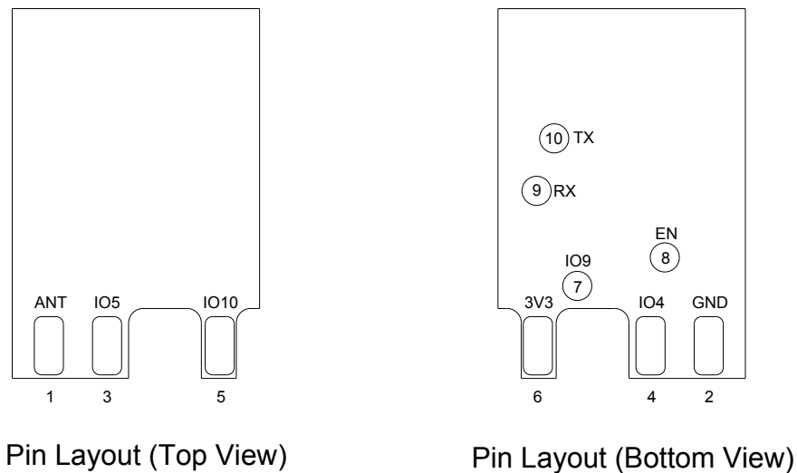
Figure 2: Pin Layout
