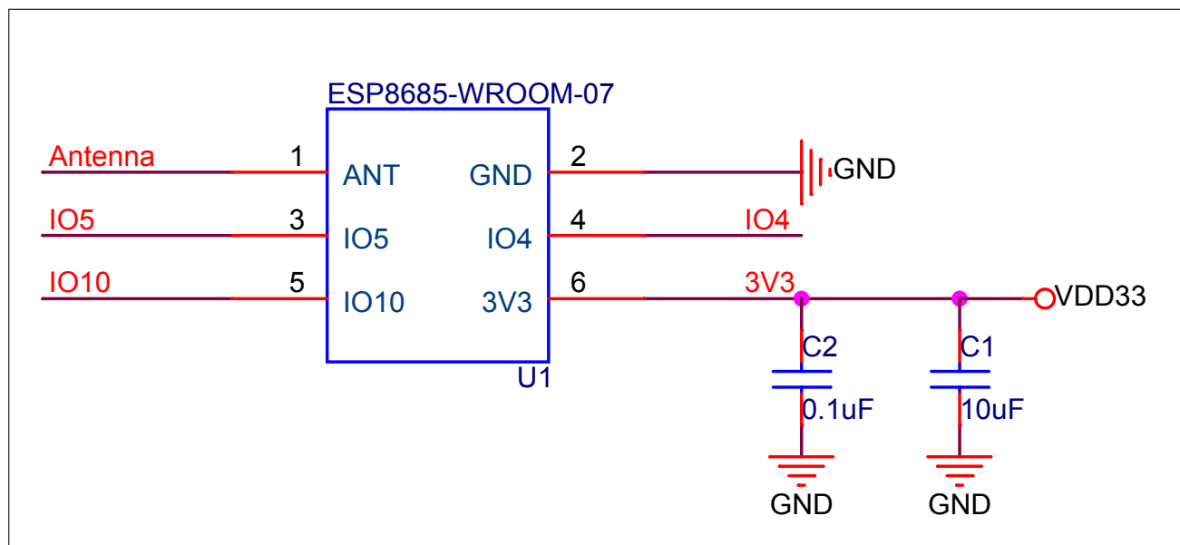
Figure 5: Peripheral Schematics
