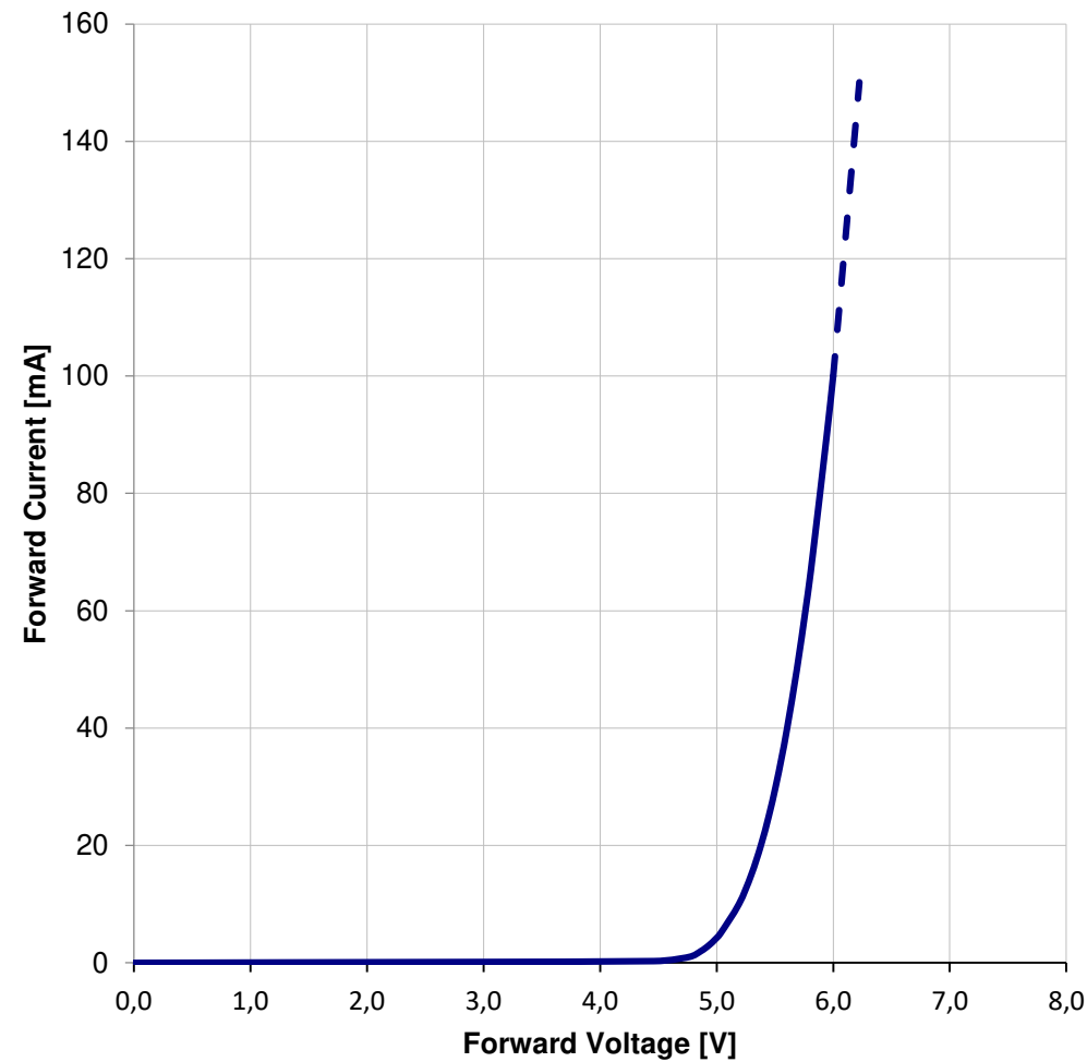
Forward Current vs. Forward Voltage:
