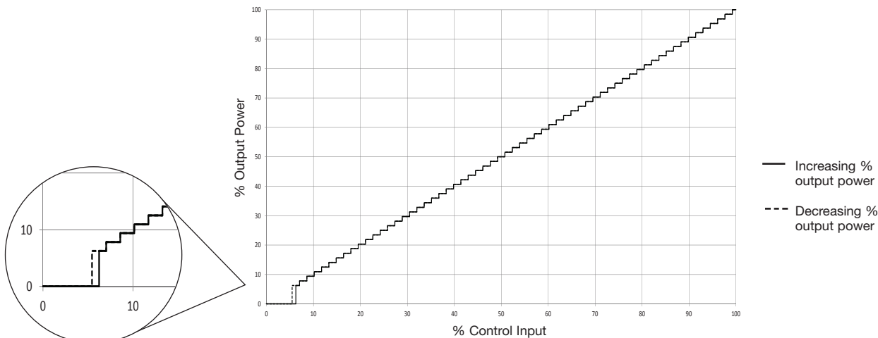
16 Full cycles switching mode: RGC...C16
