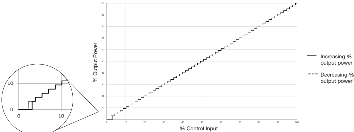
4 Full cycles switching mode: RGC...C4
