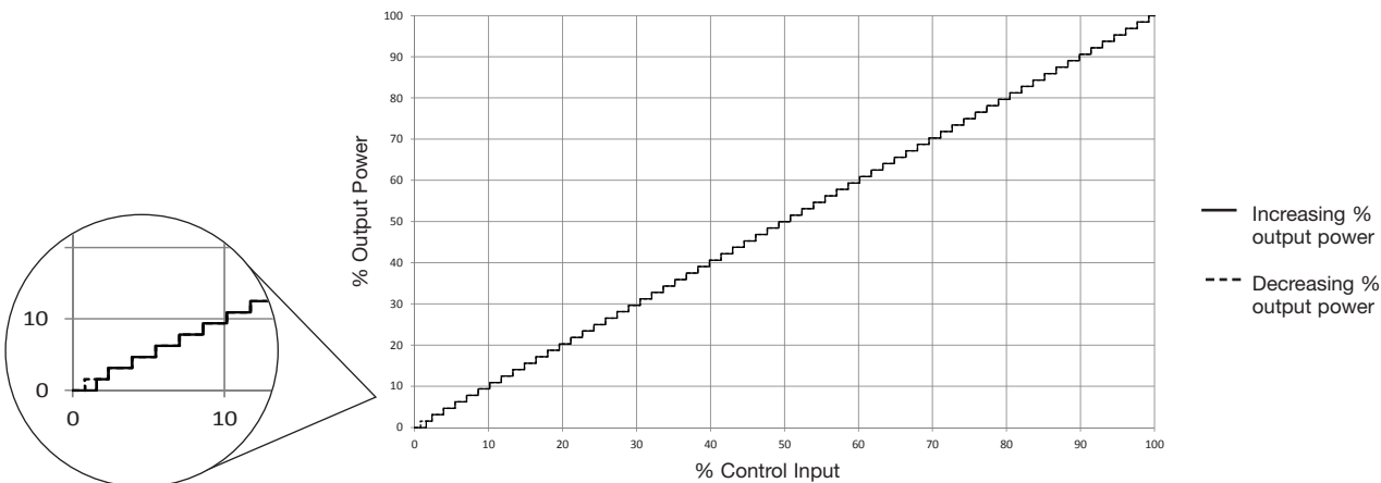
1 Full cycle switching mode: RGC...C1
