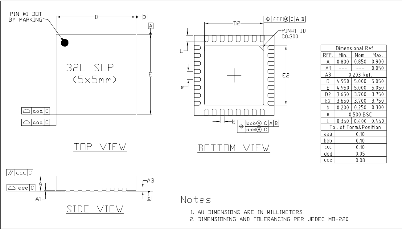
Figure 5-1. QFN32 (5×5 mm) Package
