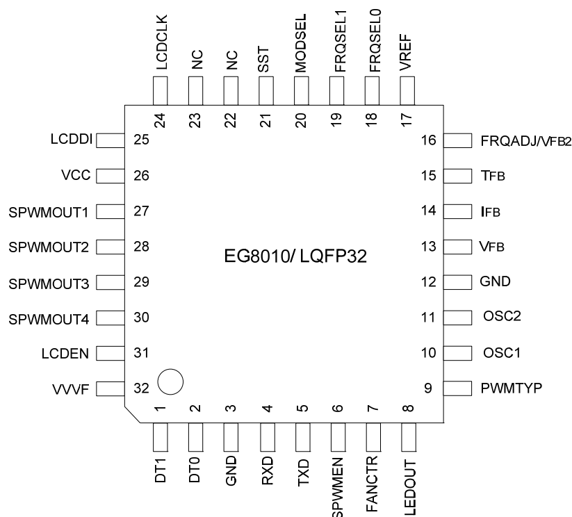
Figure 4.1EG8010 pin map
