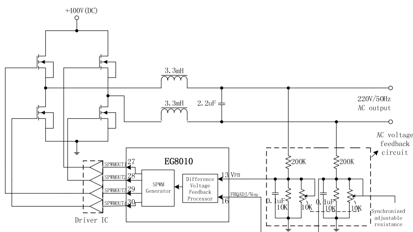
Figure 8.1cEG8010Outputvoltage feedback circuit under bipolar modulation
