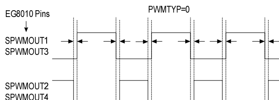
Figure 8.4a EG8010 Positive PWM output
