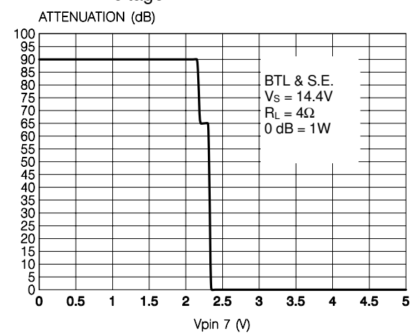
Figure 17: Stand-by Attenuation vs. Threshold Voltage
