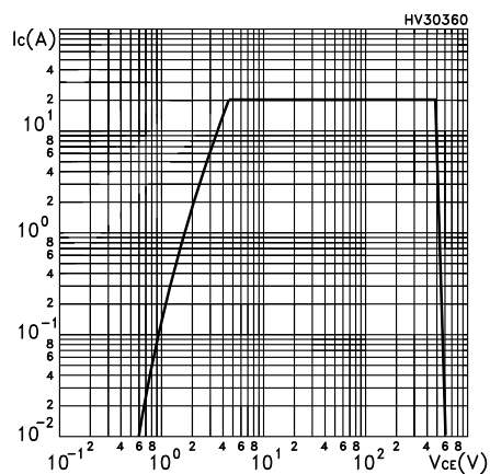
Figure 14. Turn-off SOA
