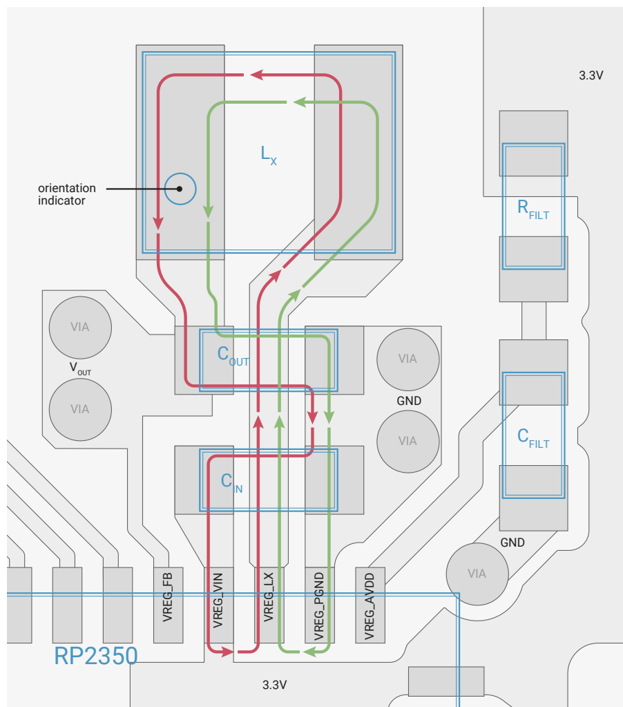
Figure 22. Regulator section of the Raspberry Pi Pico 2 PCB layout showing the high current paths for each of the regulator's switching phases. The AOTA-B201610S3R3-101-T inductor's case size is 0806 (2016 metric), the resistor and capacitors are 0402 (1005 metric)
