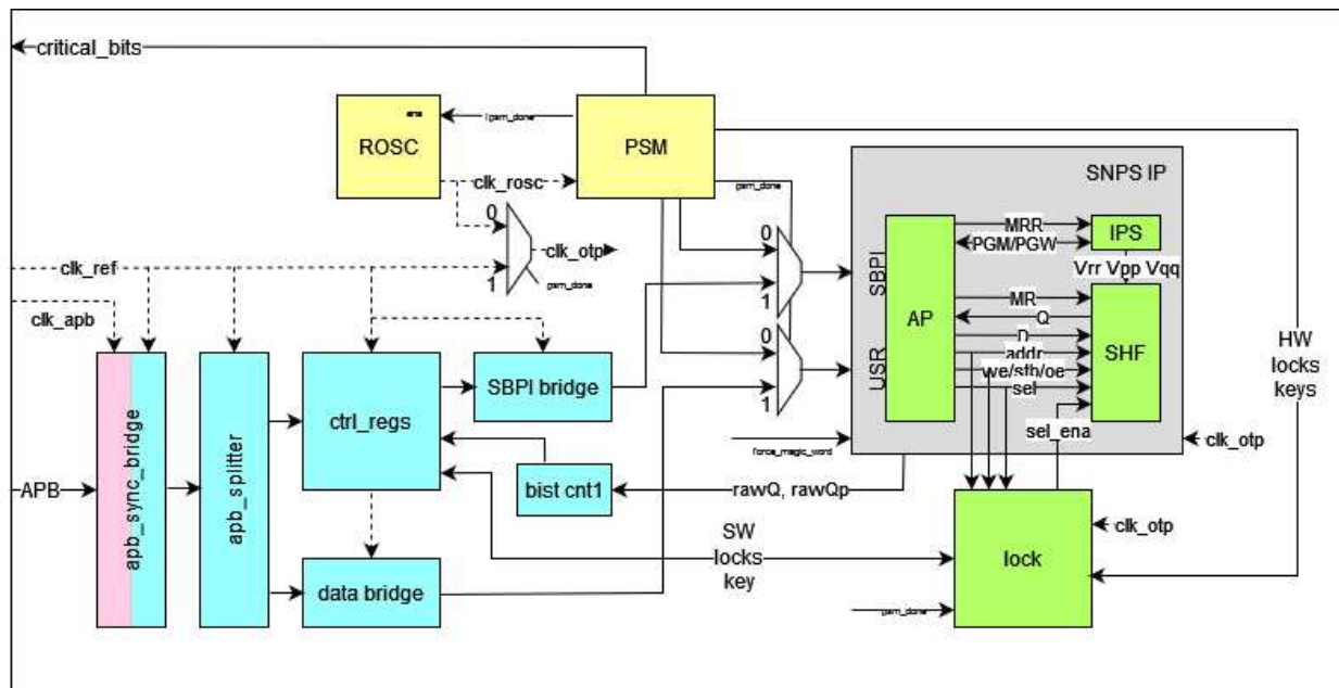
Figure 141. OTP architecture
