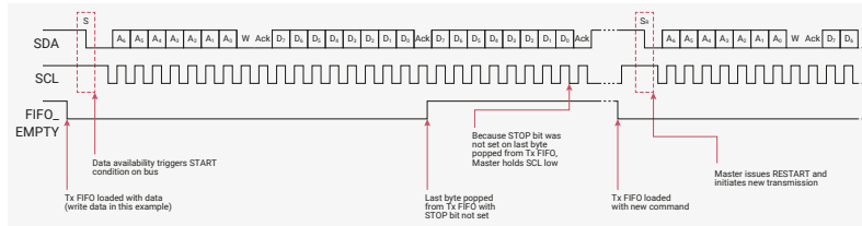
Figure 81. Master Transmitter - First Byte Loaded Into TX FIFO Allowed to Empty, Restart Bit Set
