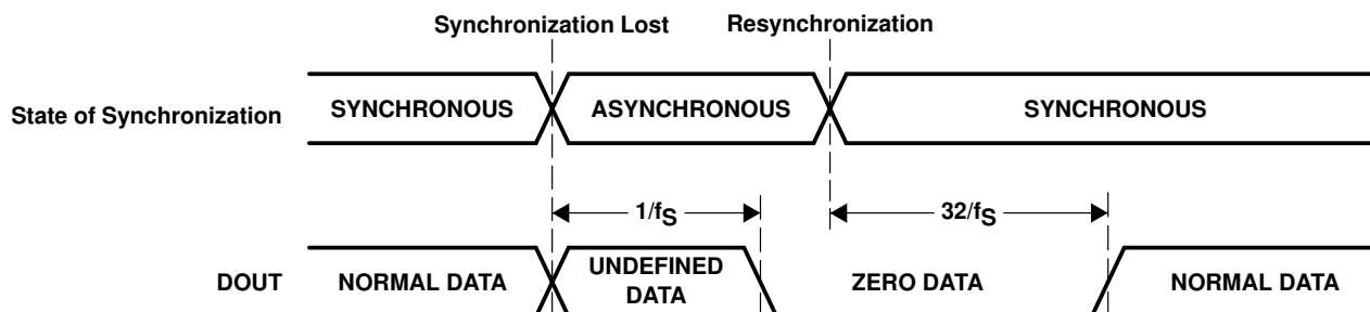
Figure 28. ADC Digital Output for Loss of Synchronization and Resynchronization
