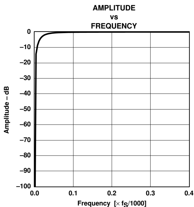
Figure 5. LCF Stopband Characteristics
