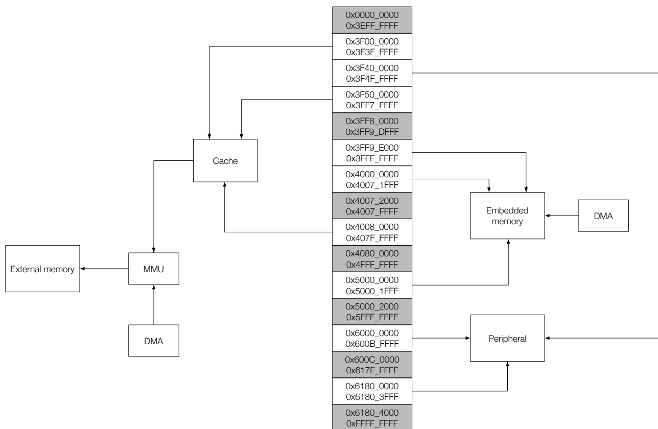
Figure 7: Address Mapping Structure
