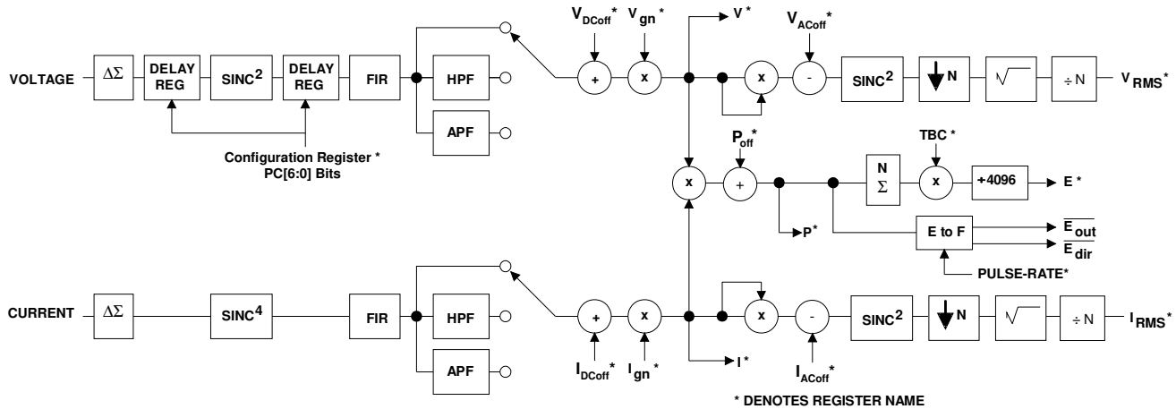
Figure 3. Data Flow.
