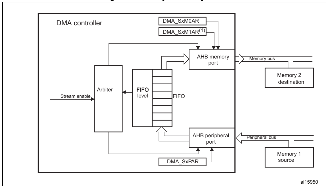
Figure 27. Memory-to-memory mode
