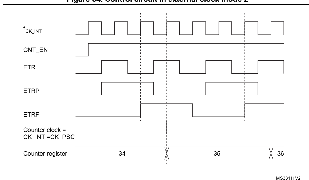
Figure 64. Control circuit in external clock mode 2
