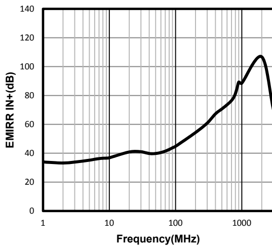
EMIRR IN+ vs. Frequency
