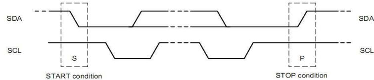
Figure 7: Schematic start and stop conditions
