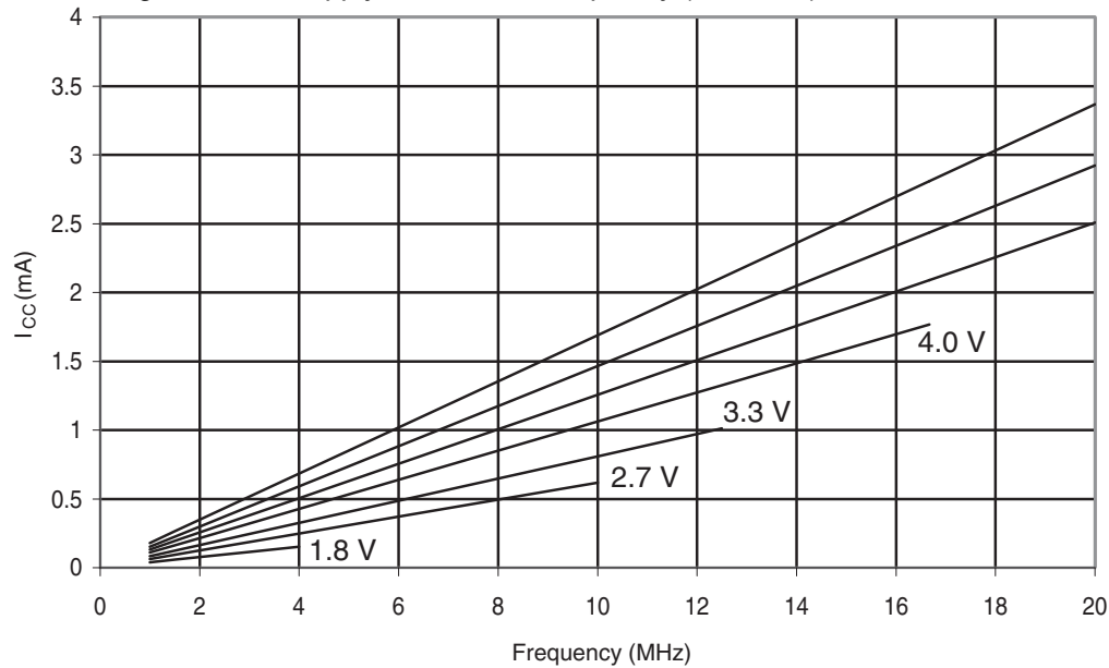
Figure 30-289. ATmega328: Idle Supply Current vs. Frequency (1-20MHz)
