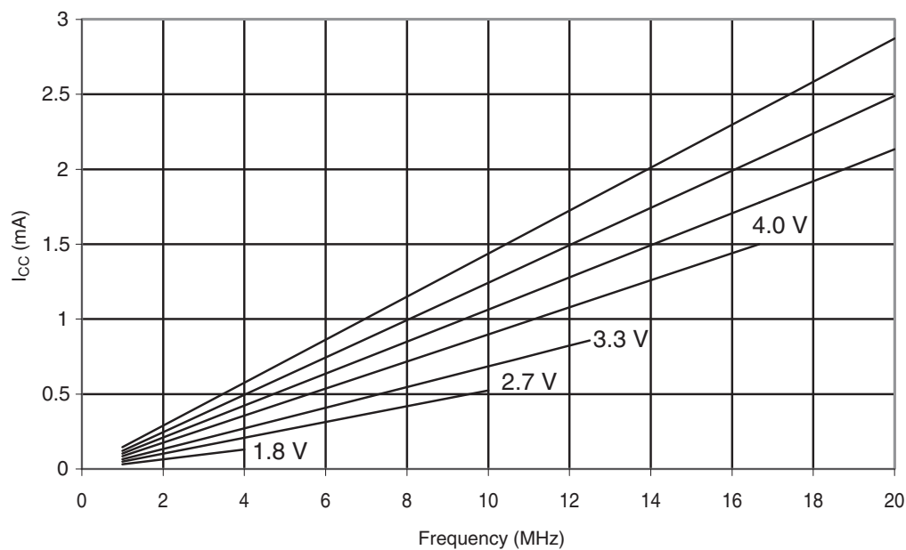
Figure 30-375. ATmega328P: Reset Supply Current vs. Frequency (1 - 20MHz)
