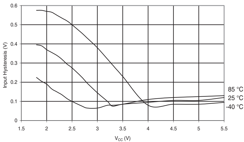
Figure 30-124. ATmega88A: Reset Pin Input Hysteresis vs. V_{CC}
