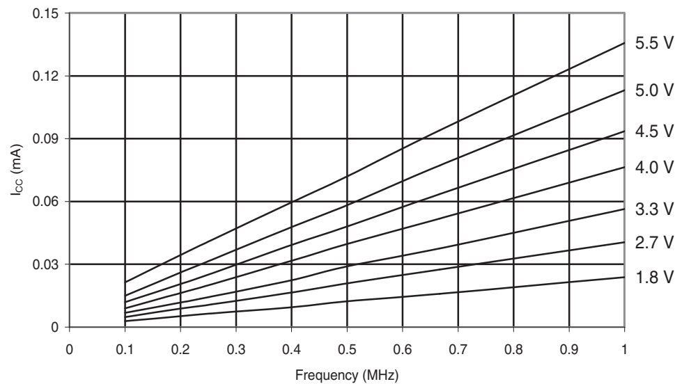
Figure 30-194.ATmega168A: Idle Supply Current vs. Low Frequency (0.1-1.0MHz)
