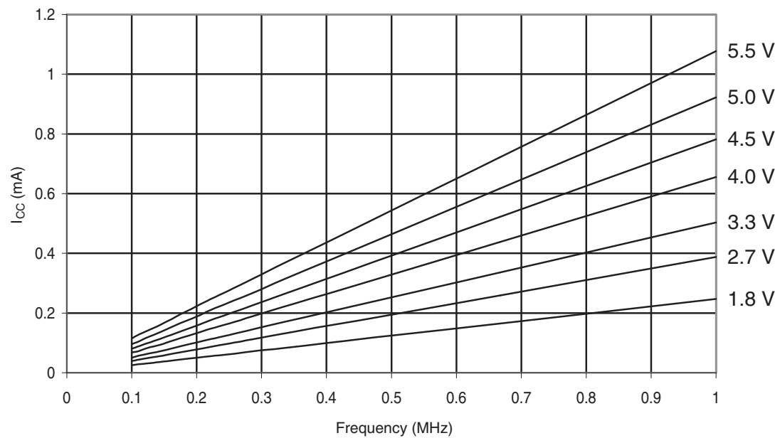
Figure 30-330.ATmega328P: Active Supply Current vs. Low Frequency (0.1-1.0MHz)
