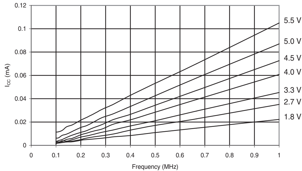
Figure 30-139.ATmega88A: Reset Supply Current vs. Low Frequency (0.1 - 1.0MHz)
