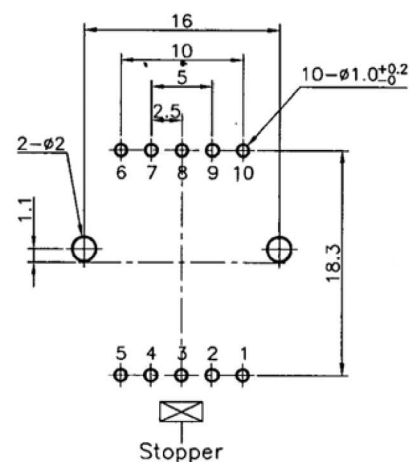
P.C.B MOUNTING DETAIL
