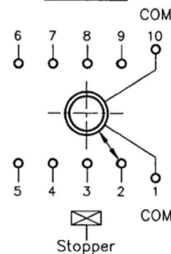
SCHEMATIC
