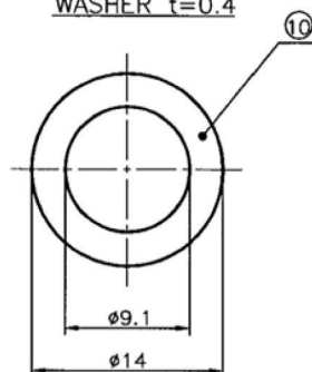
WASHER t=0.4
