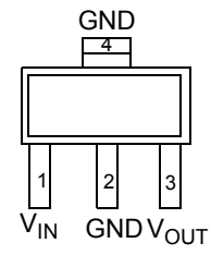
3-Pin SOT-223
