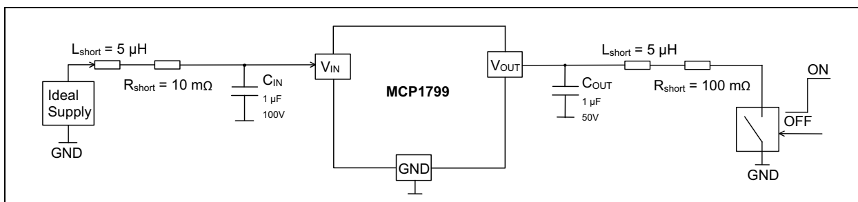
FIGURE 4-2: Short Circuit Test Set-Up.
