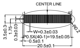
DETAIL A (3:1)
