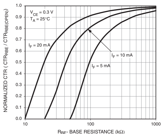
Figure 7. CTR vs. R_BE (Saturated)
