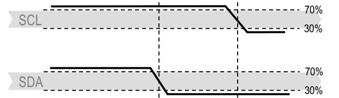
Figure 13 Start Transmit State (S) - When SCL is at high level, SDA is converted from high level to low level. The start state is a special bus state controlled by the main engine, indicating the start of slave machine transit (after Start, BUS is generally considered to be in a busy state).
