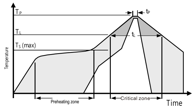
Figure 9 JEDEC Standard welding procedure diagram. T_p \leq 260^\circ\text{C} , t_p \leq 30 sec, lead-free welding. T_L < 220^\circ\text{C} , t_L < 150 sec, The rate of temperature rise and fall during welding shall be < 5^\circ\text{C}/\text{sec} .
