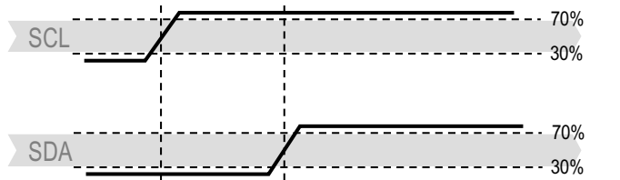
Figure 14 Stop Transmit State (P) - When the SCL is at high level, the SDA line is converted from low level to high level. Stop state is a special bus state controlled by the main engine, indicating the end of slave machine transmit (after Stop, BUS is generally considered to be in idle state).
