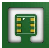
Figure 10 AHT20 top view of printing circuit board. The design of milling slit can minimize heat transfer.
