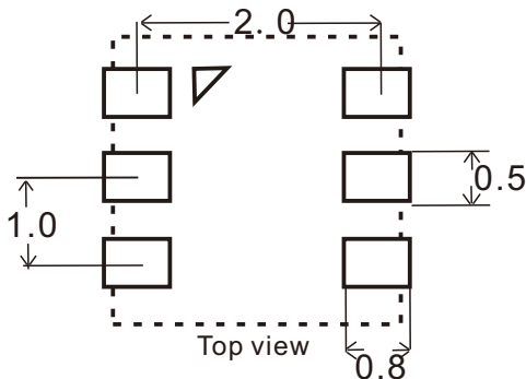
Figure 8. Recommended design size of AHT20 PCB (mm) and the outer part with dotted line is the outer dimension of SMD package.
