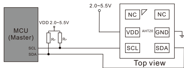
Figure 11 Typical application circuits including pull-up resistance RP and decoupling capacitance between VDD and GND.
