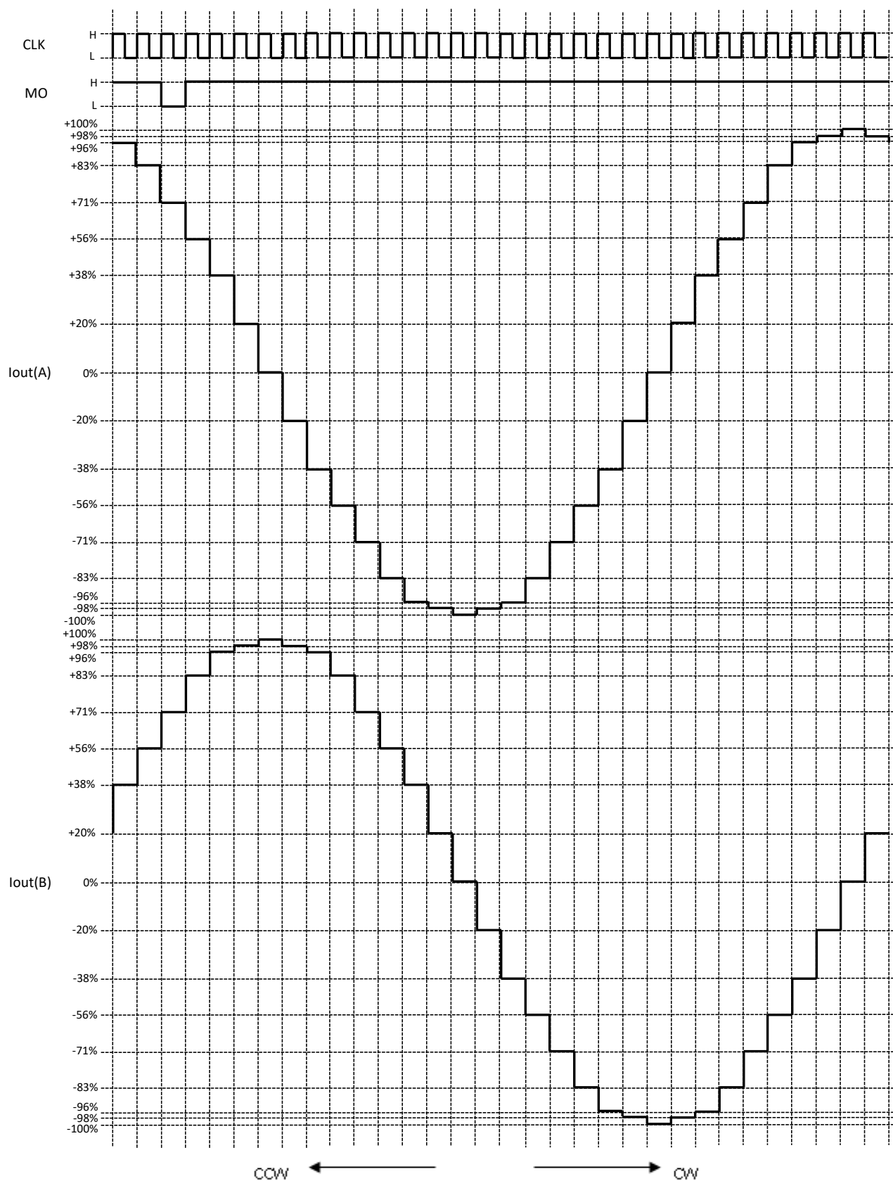
Figure 6.5 1/8 step resolution
