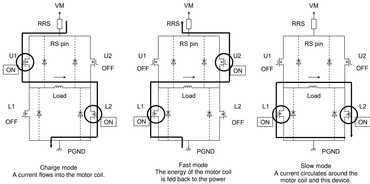
Figure 6.15 Output transistor function mode
