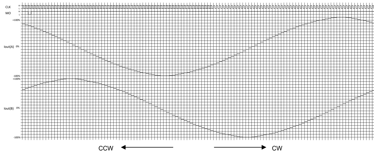
Figure 6.7 1/32 step resolution
