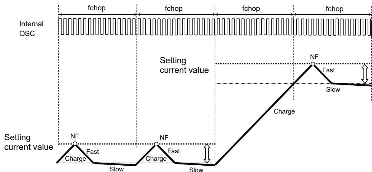
Figure 6.12 When Charge period is more than 1 fchop cycle
