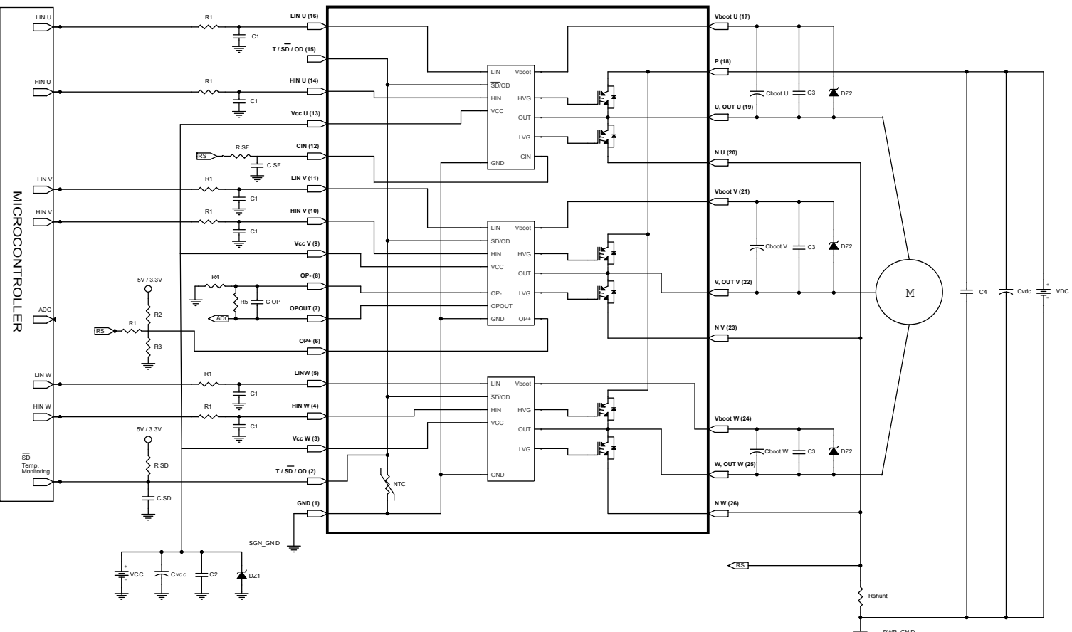
Figure 12. Application circuit example
