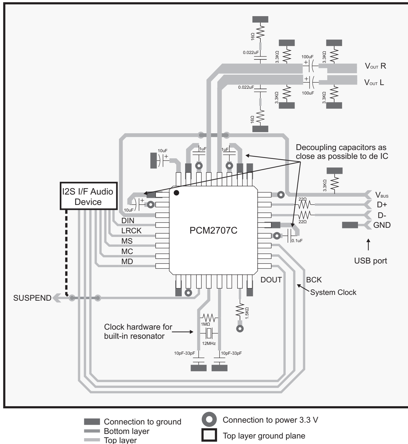
Figure 40. Layout Example 3
