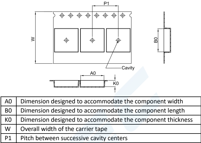
TAPE DIMENSIONS
