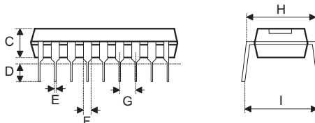
Fig2. 1/2 Lead Packages
