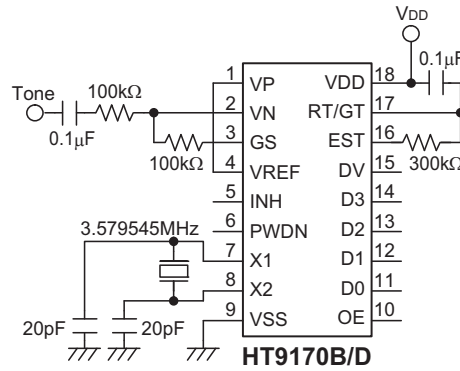
Figure 1. Test circuit
