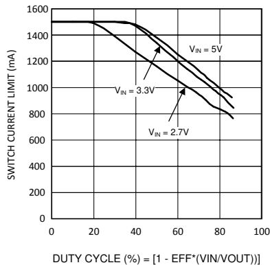
Figure 26. Switch Current Limit vs Duty Cycle - "X"
