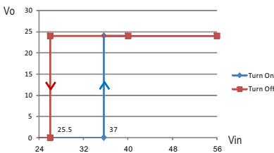
RSD-60H-24
