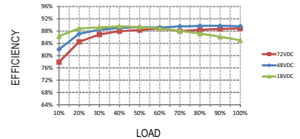
RSD-60H-3.3
