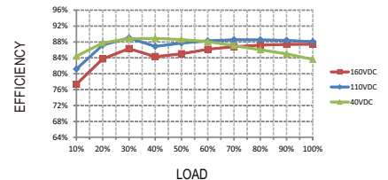
RSD-60H-24
