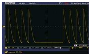
ISO7637-2 TP3B
