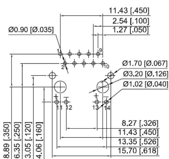
10 Pins, w/ LED For 100 PoE/1000/2.5G/5G Base-T
