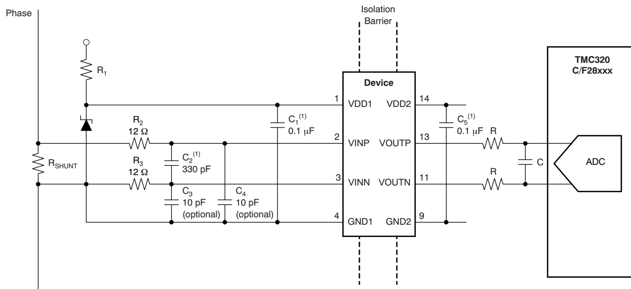
Figure 33. Shunt-Based Current Sensing with the AMC1200
