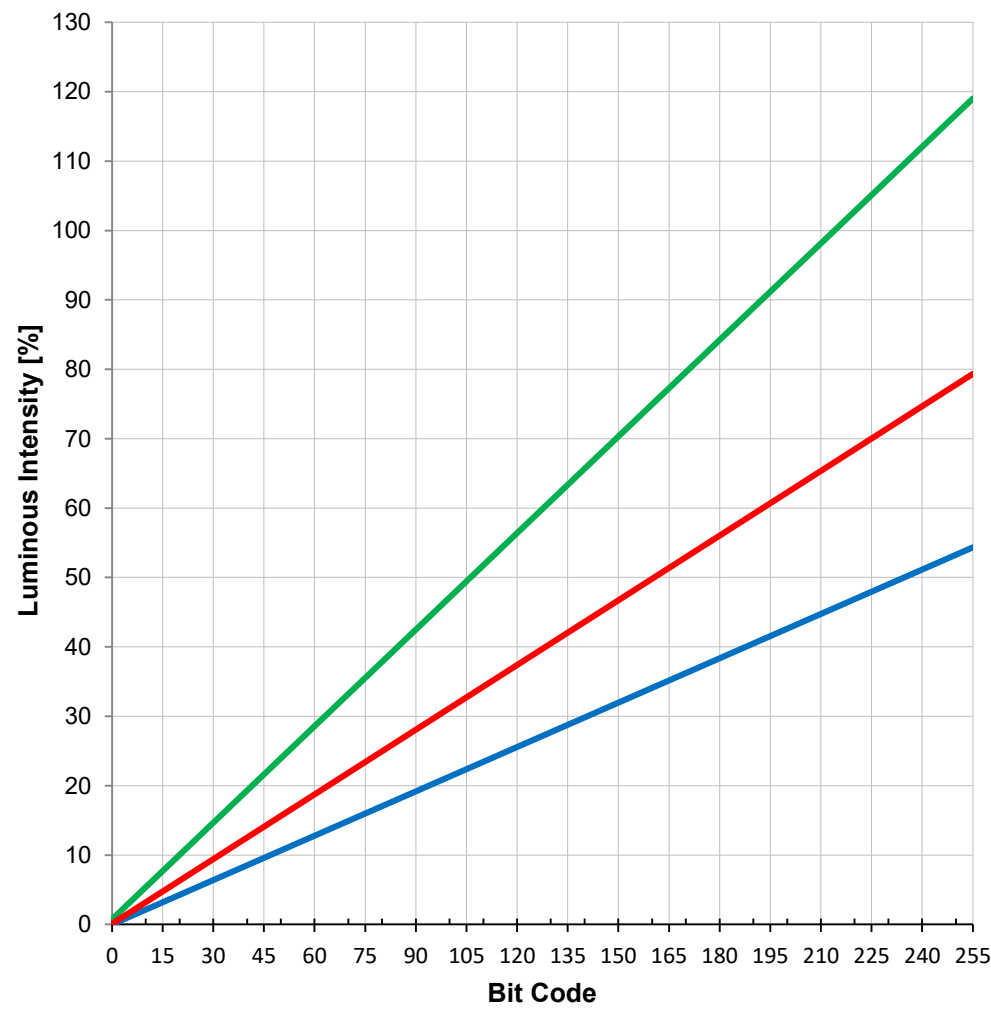
Typical luminous intensity vs. Bit Code:
