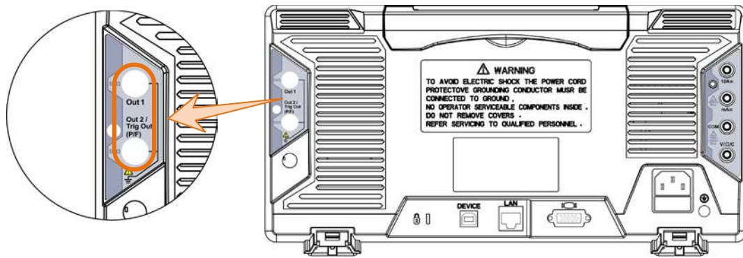
Figure 4-1 Generator Output Ports
