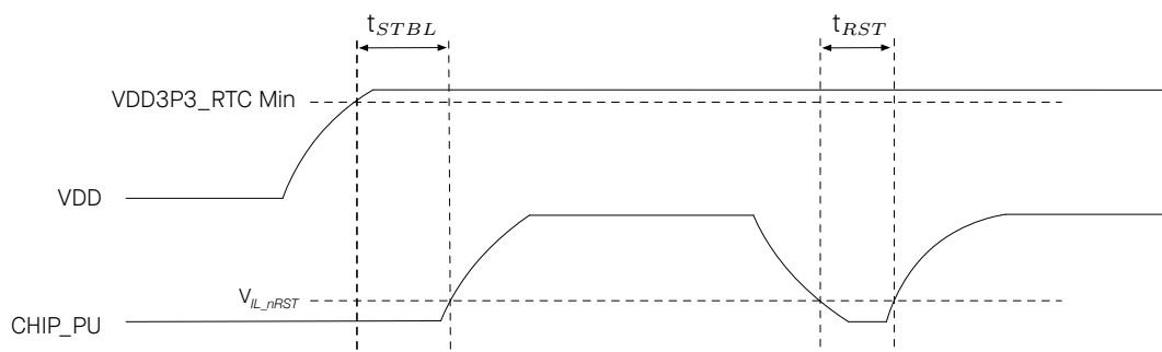
Figure 6: Visualization of Timing Parameters for Power-up and Reset
