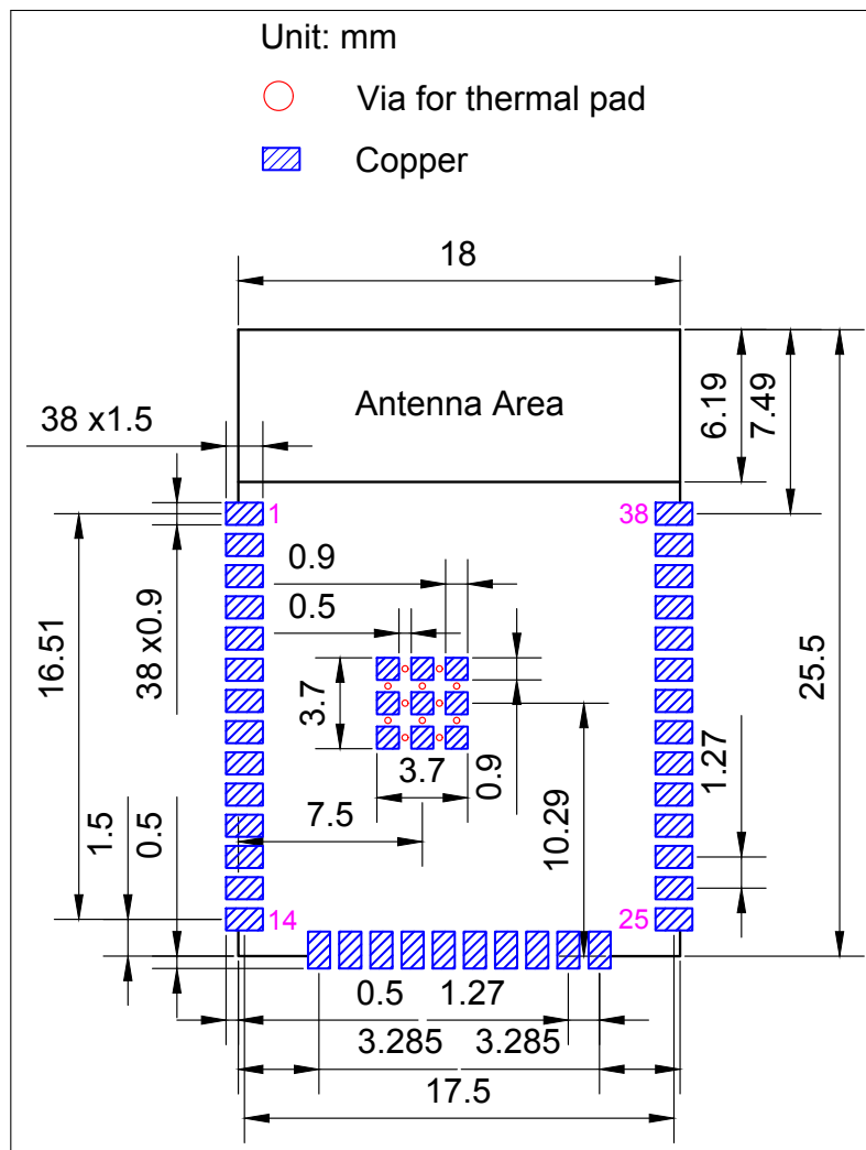
Figure 13: ESP32-WROOM-32E Recommended PCB Land Pattern
