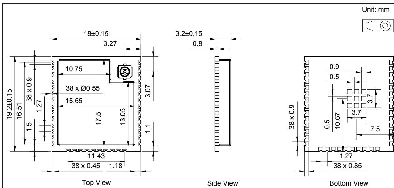
Figure 11: ESP32-WROOM-32UE Physical Dimensions
