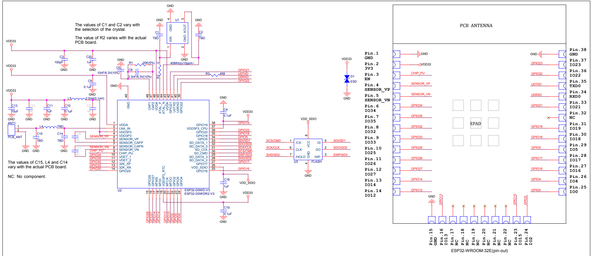
Figure 7: ESP32-WROOM-32E Schematics
