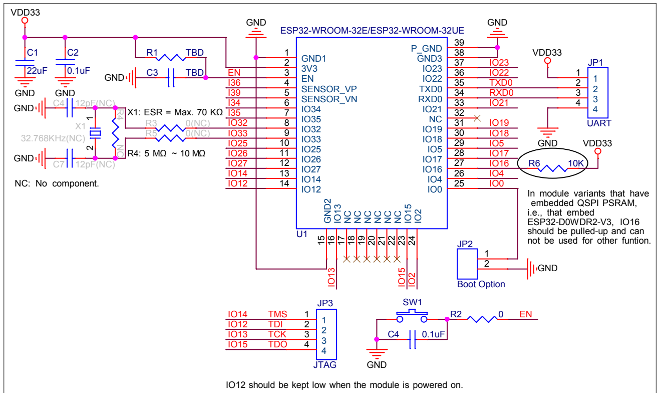
Figure 9: Peripheral Schematics
