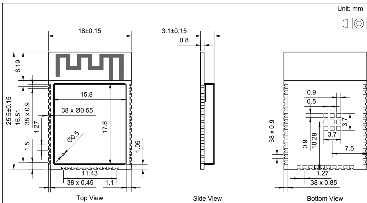
Figure 10: ESP32-WROOM-32E Physical Dimensions
