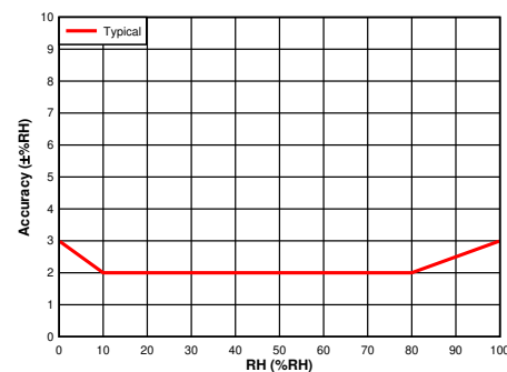
RH Accuracy ( T_A = 30^\circ\text{C} )
