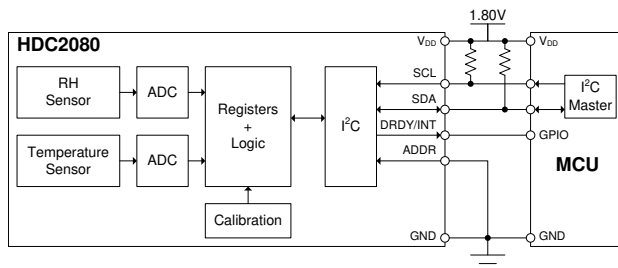
Typical Application
