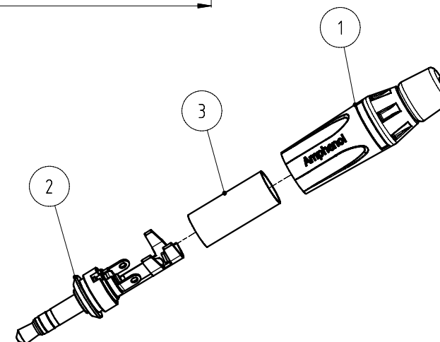
EXPLORED VIEW ( 1 : 1 )
