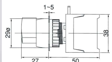
LRS22-1/O 0-1 Spring return LRS22-1/C 1-0
