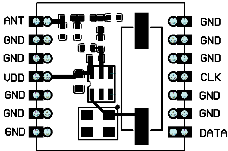
RFM119S. Pin Diagram
