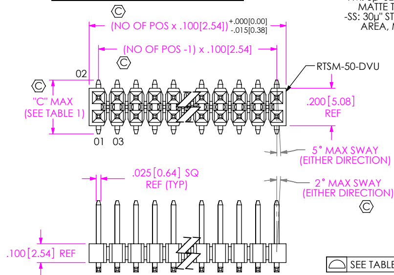
FIG 1 TSM-1XX-XX-XXX-DV SHOWN
