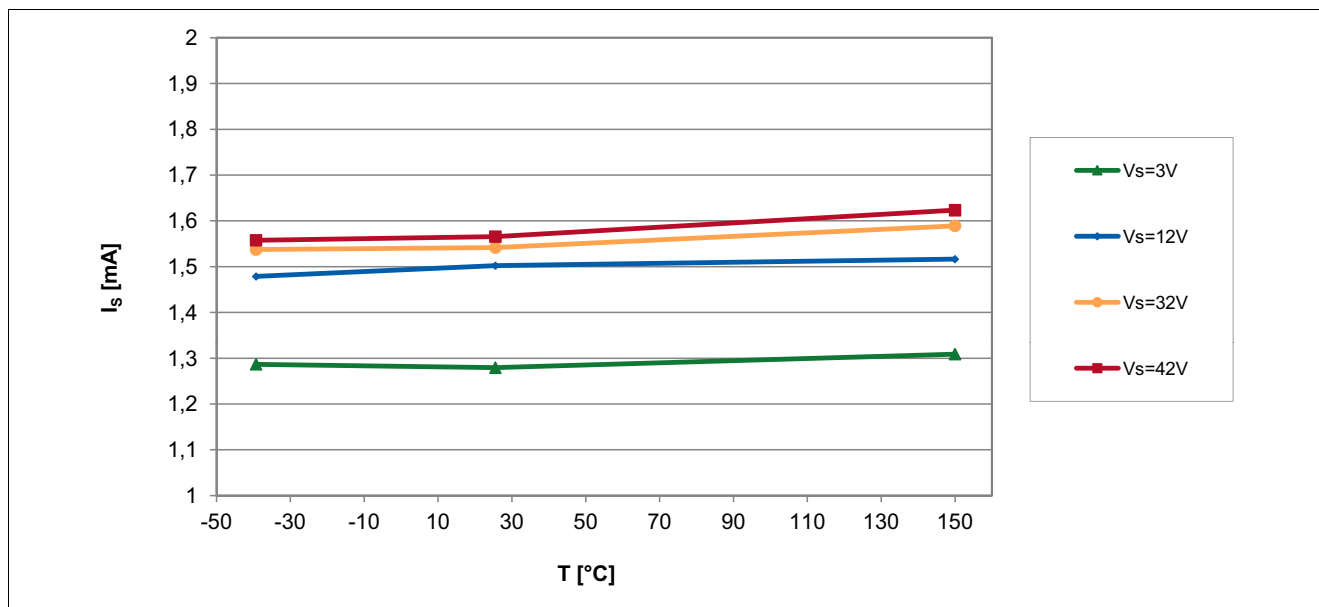
Figure 6-3 Supply Current of the TLE4961-3L over Temperature
