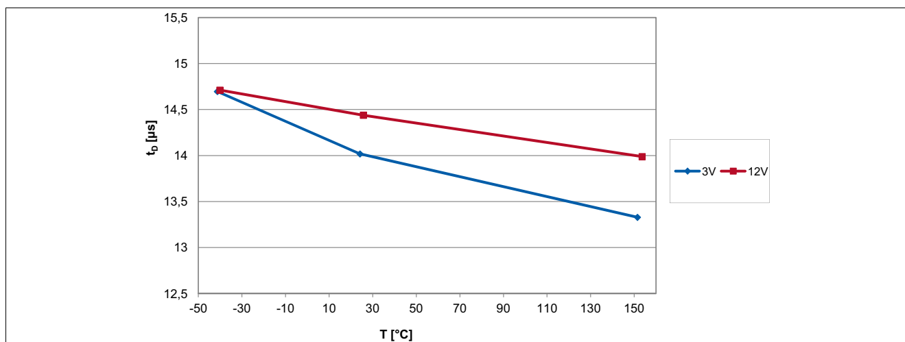
Figure 6-2 Signal Delay Time of the TLE4961-3L over Temperature
