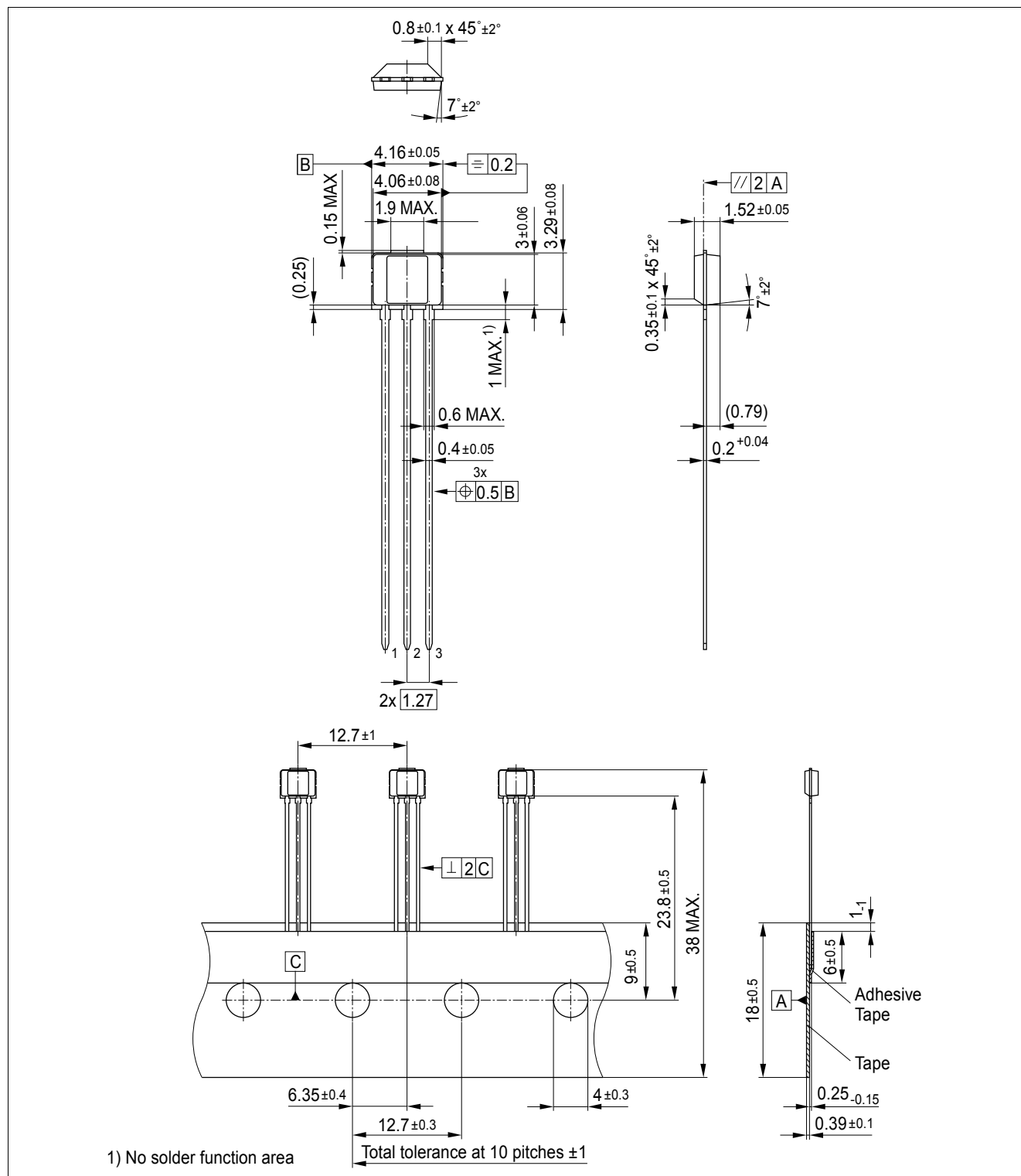
Figure 4-1 PG-SSO-3-2 Package Outline (All Dimensions in mm)
