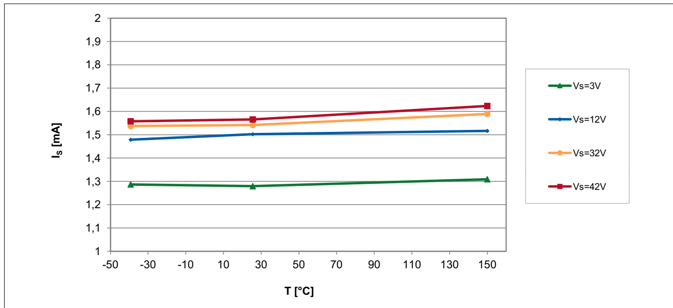
Figure 6-3 Supply Current of the TLE4961-1L over Temperature
