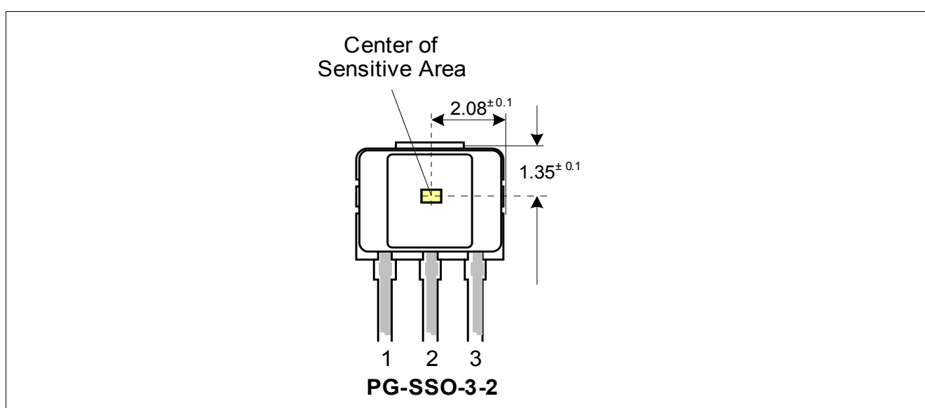
Figure 2-1 Pin Configuration and Center of Sensitive Area
