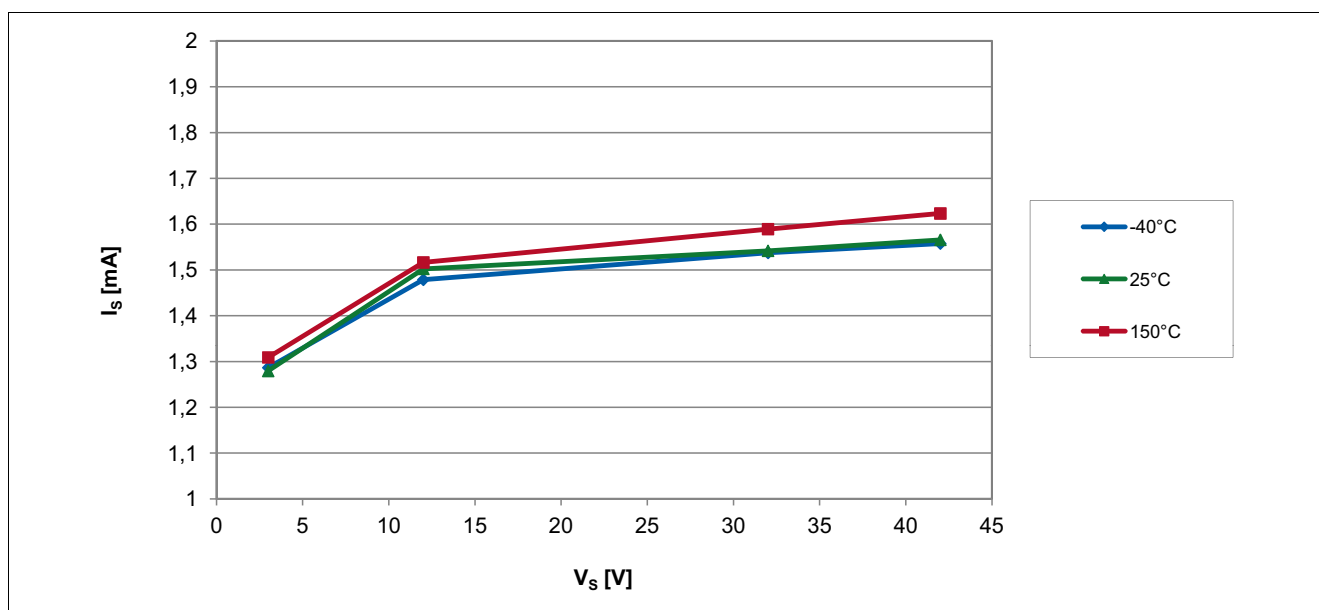
Figure 6-4 Supply Current of the TLE4961-1L over Supply Voltage
