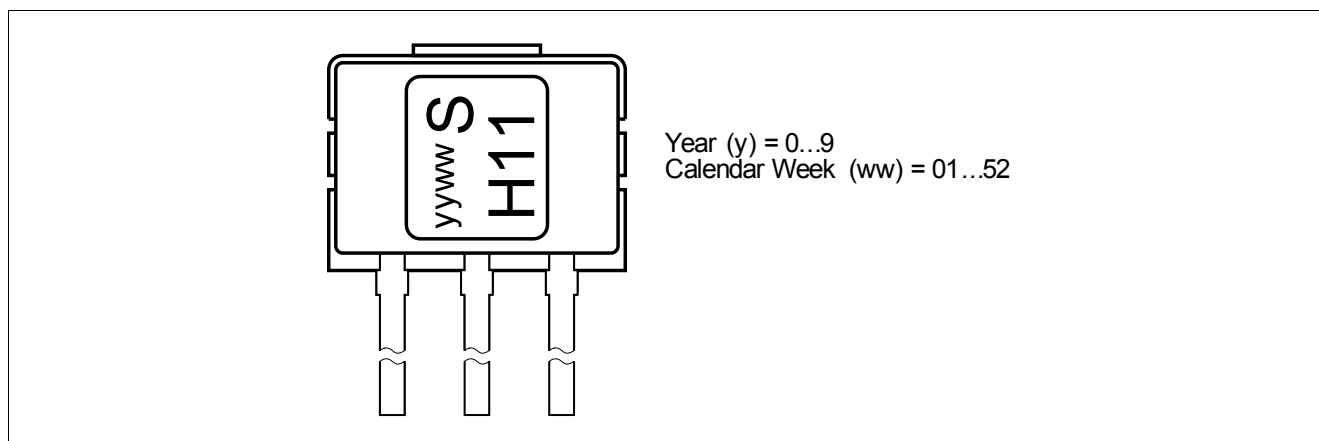
Figure 4-3 Marking of TLE4961-1L
