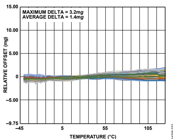
Figure 32. ADXL355 Y-Axis Zero g Offset Relative to 25°C vs. Temperature
