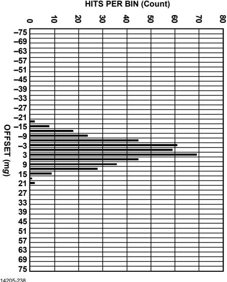
Figure 38. ADXL355 Zero g Offset Histogram at 25°C, Y-Axis
