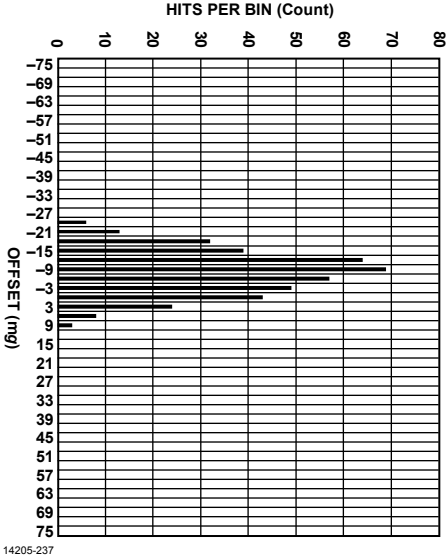
Figure 37. ADXL355 Zero g Offset Histogram at 25°C, X-Axis
