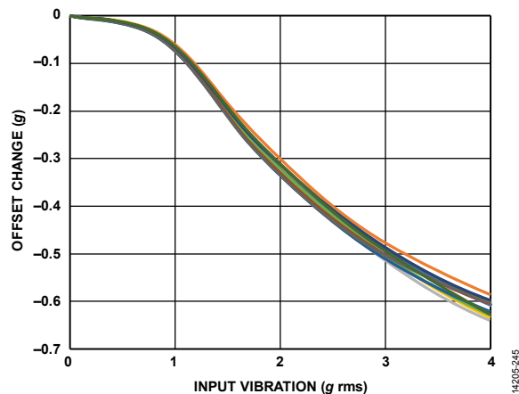
Figure 45. ADXL355 Vibration Rectification Error (VRE), Z-Axis Offset from +1 g, \pm 2 g Range, Z-Axis Orientation = +1 g
