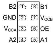
Figure 4-4. DTT Package, 8-Pin SOP (Top View)
