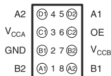
Figure 4-1. YZP Package, 8-Pin DSBGA (Bottom View)
