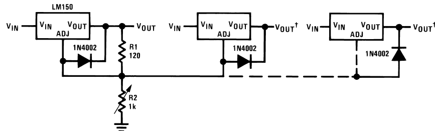
Figure 35. Tracking Preregulator
