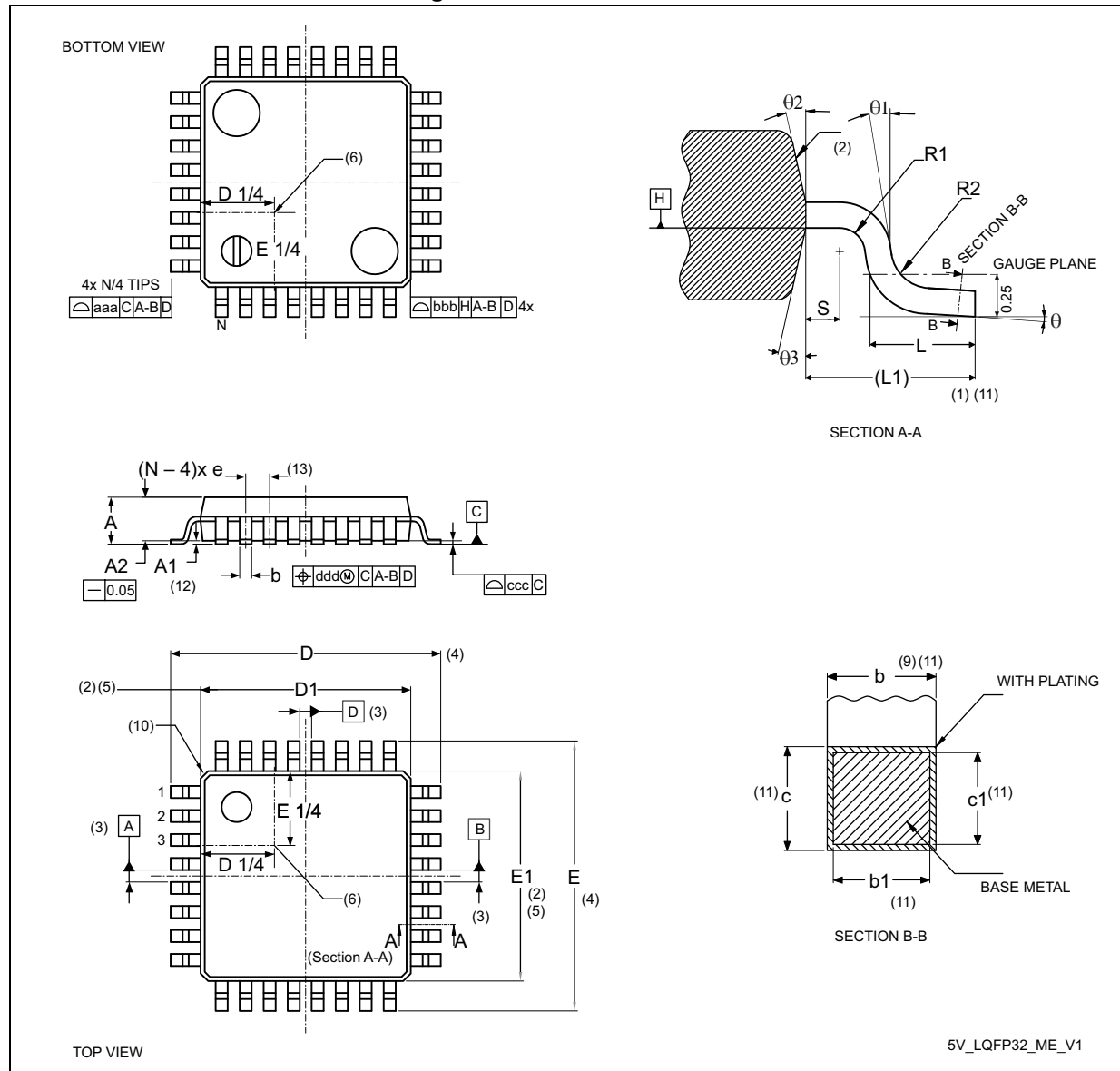
Figure 33. LQFP32 - Outline
