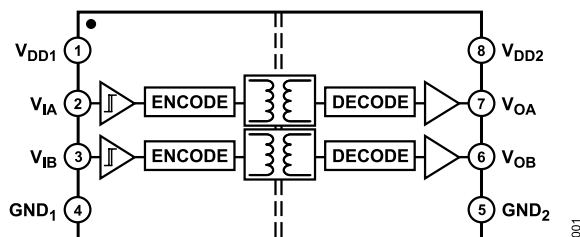
Figure 1. ADuM1200 Functional Block Diagram
