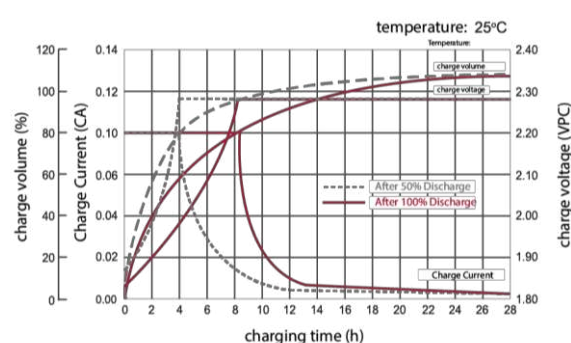
CHARGE CHARACTERISTIC CURVE FOR CYCLE USE
