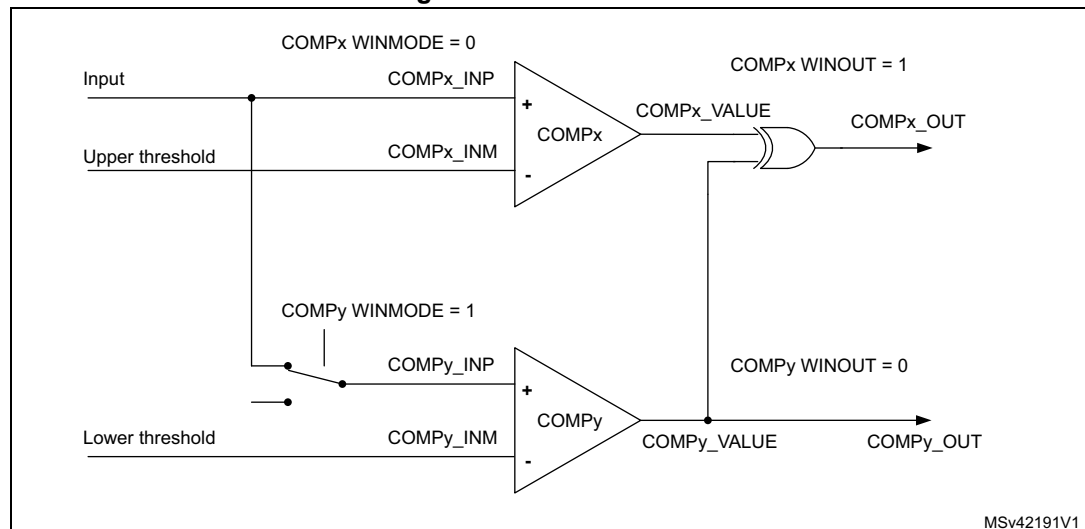
Figure 69. Window mode
