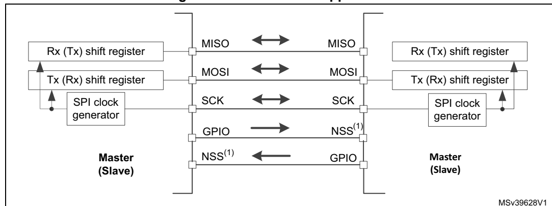
Figure 360. Multimaster application
