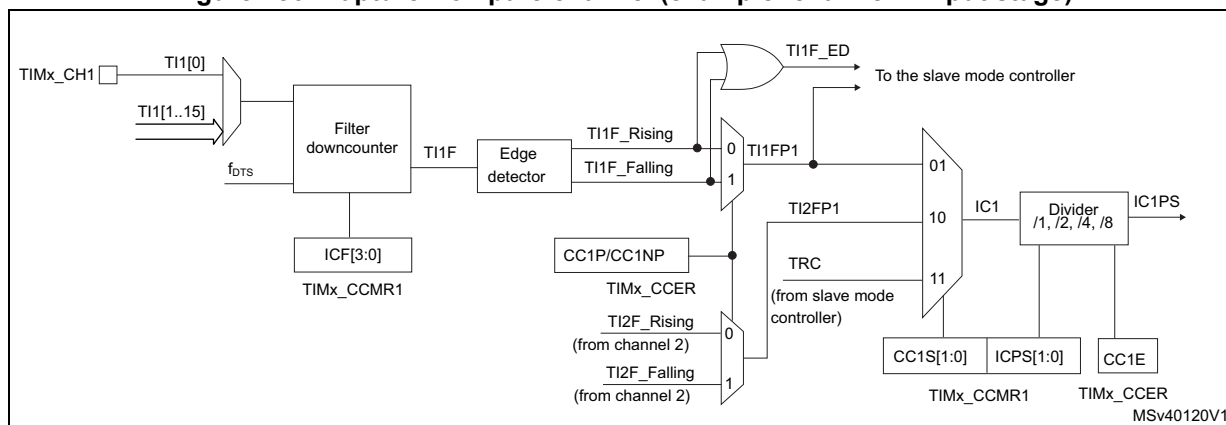
Figure 186. Capture/Compare channel (example: channel 1 input stage)
