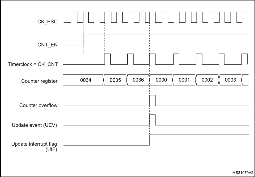
Figure 225. Counter timing diagram, internal clock divided by 2
