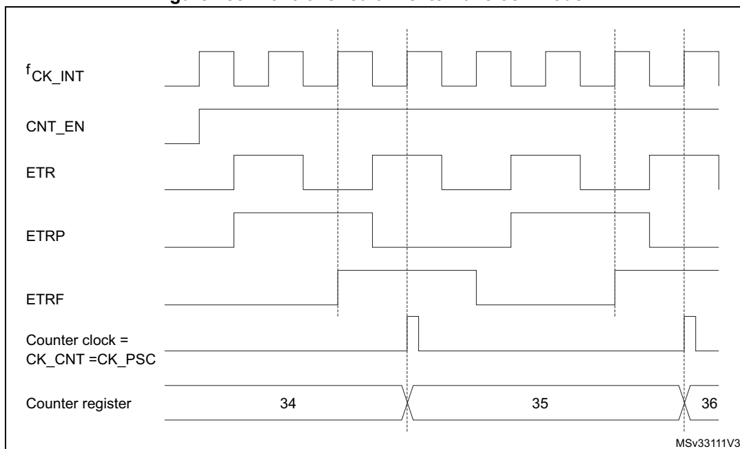
Figure 185. Control circuit in external clock mode 2
