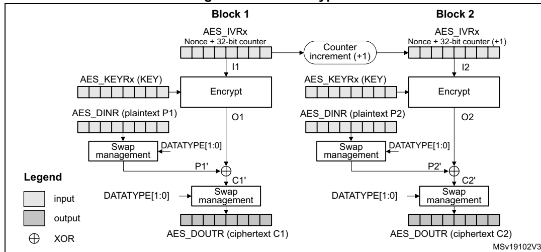
Figure 90. CTR encryption
