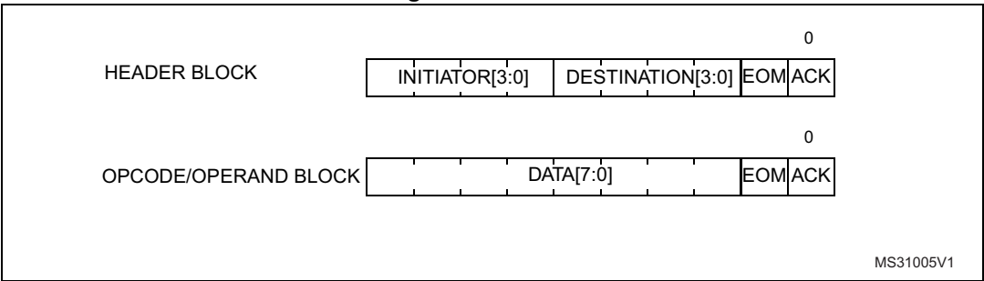
Figure 417. Blocks
