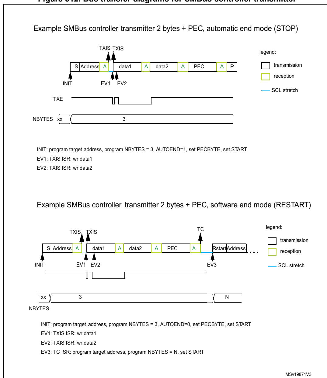
Figure 312. Bus transfer diagrams for SMBus controller transmitter
