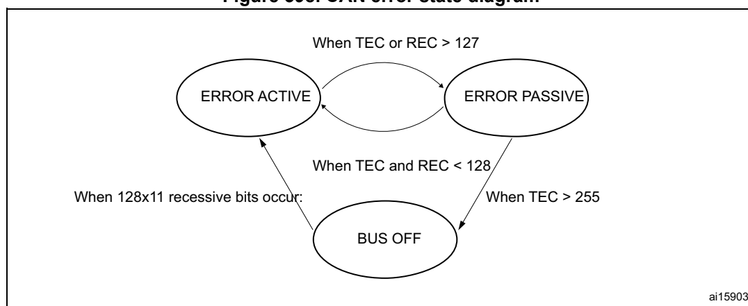
Figure 398. CAN error state diagram
