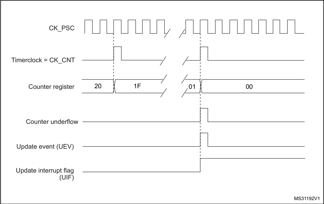
Figure 178. Counter timing diagram, internal clock divided by N
