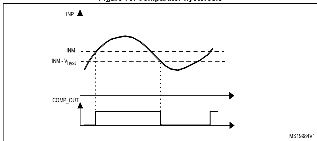
Figure 70. Comparator hysteresis
