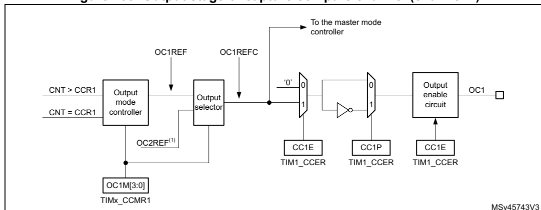
Figure 233. Output stage of capture/compare channel (channel 1)
