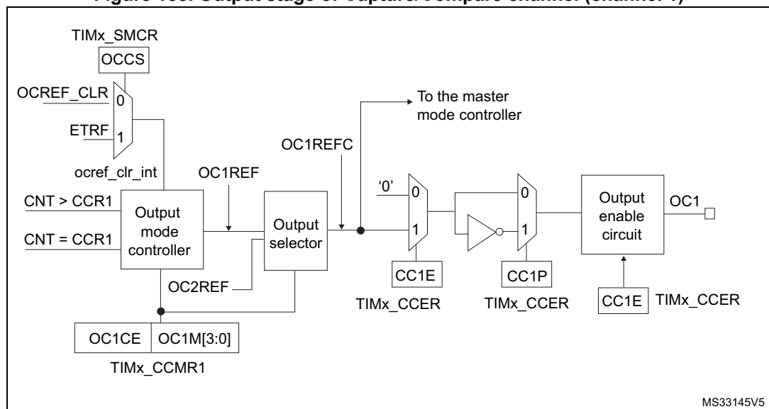
Figure 188. Output stage of Capture/Compare channel (channel 1)
