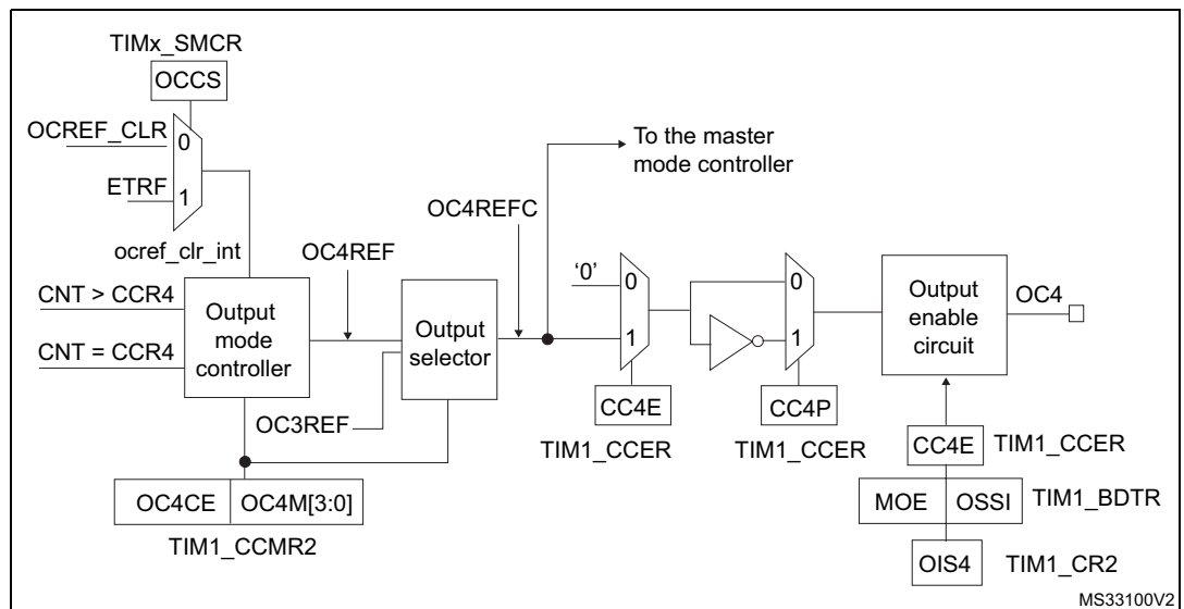
Figure 132. Output stage of capture/compare channel (channel 4)
