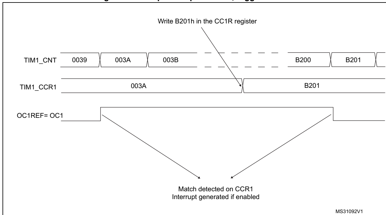
Figure 190. Output compare mode, toggle on OC1
