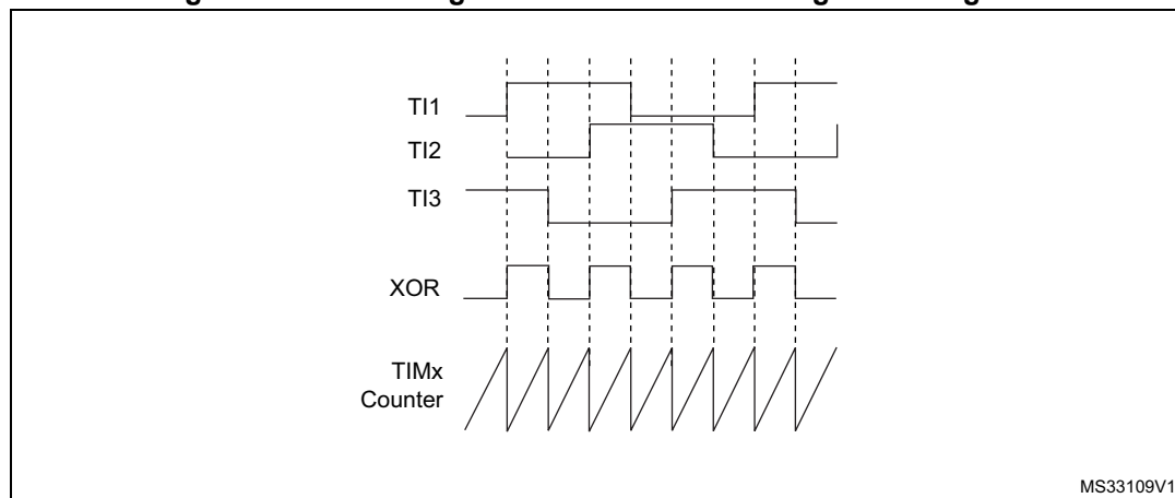
Figure 155. Measuring time interval between edges on 3 signals
