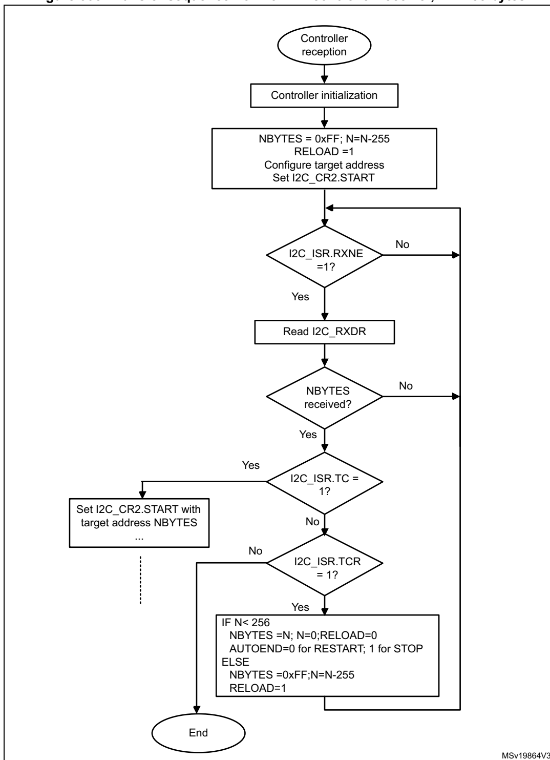
Figure 305. Transfer sequence flow for I2C controller receiver, N &gt; 255 bytes
