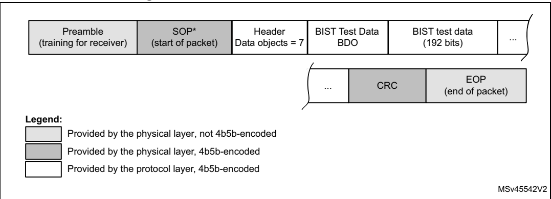
Figure 411. BIST test data frame
