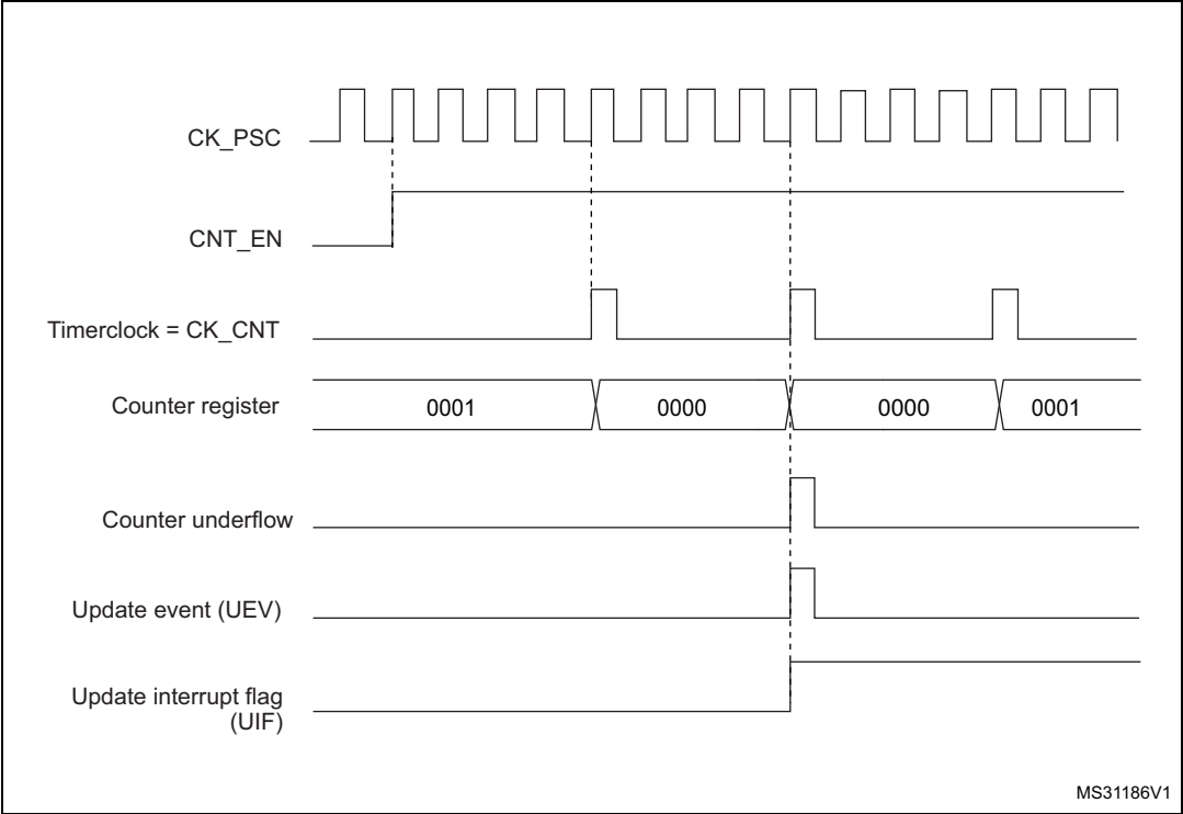
Figure 112. Counter timing diagram, internal clock divided by 4
