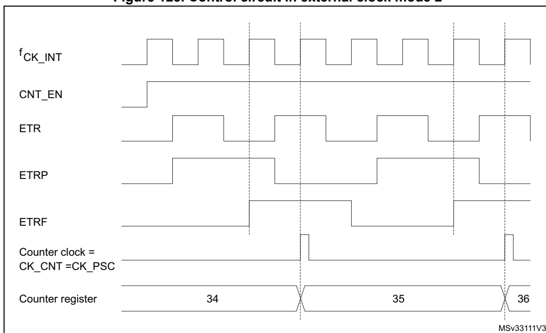
Figure 128. Control circuit in external clock mode 2
