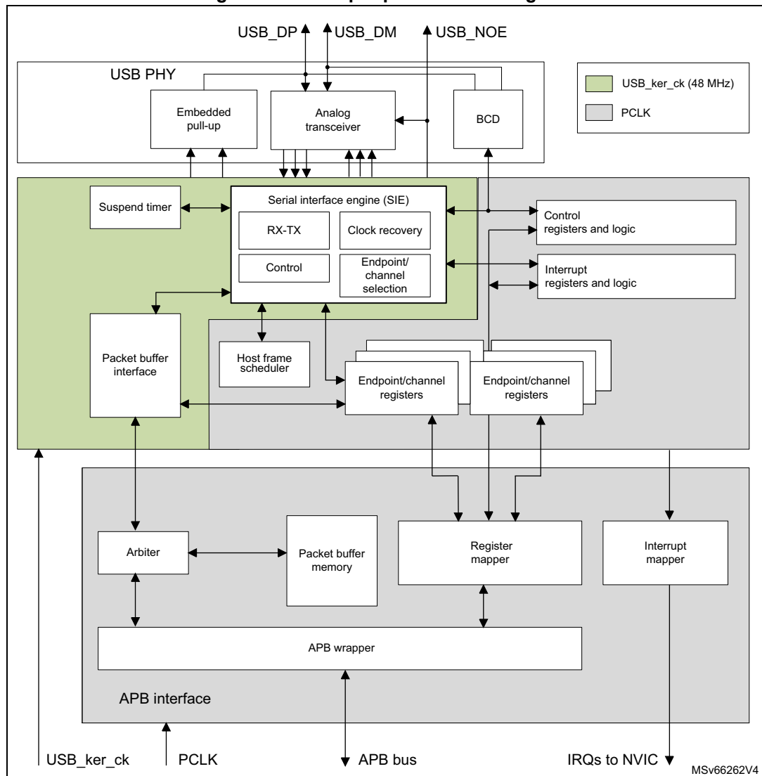
Figure 402. USB peripheral block diagram
