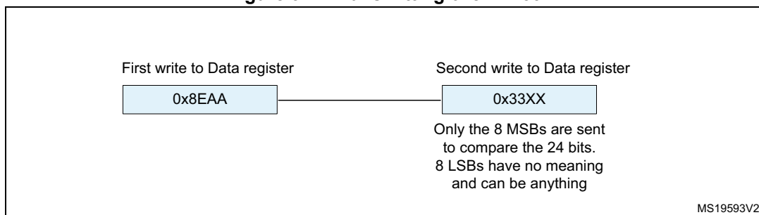
Figure 374. Transmitting 0x8EAA33
