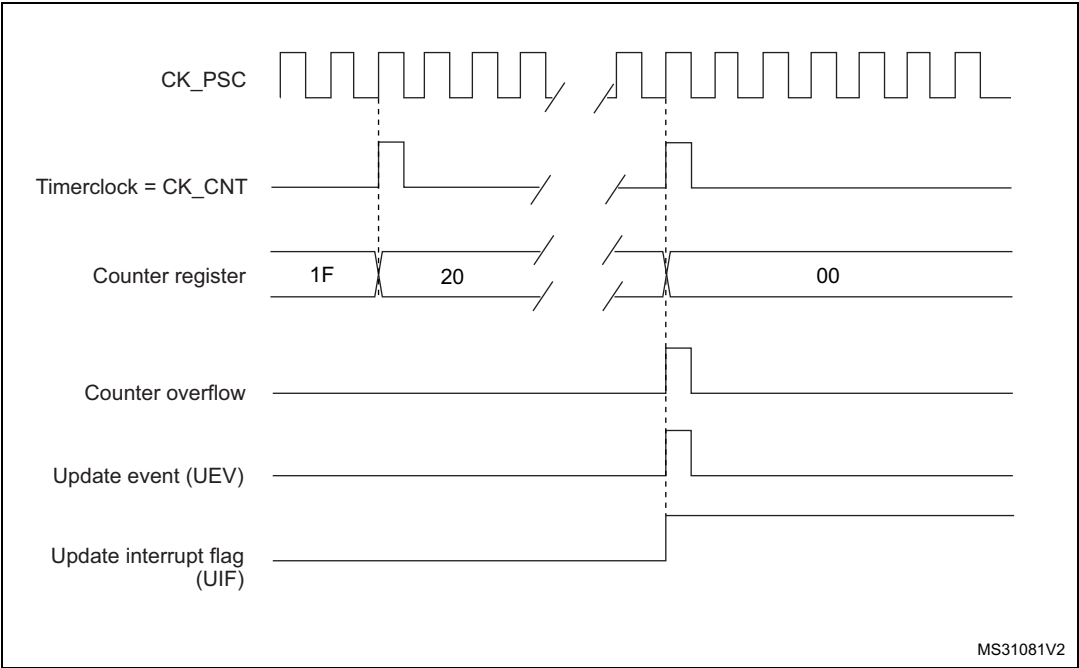
Figure 227. Counter timing diagram, internal clock divided by N
