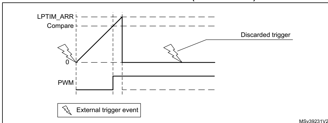
Figure 274. LPTIM output waveform, Single counting mode configuration and Set-once mode activated (WAVE bit is set)
