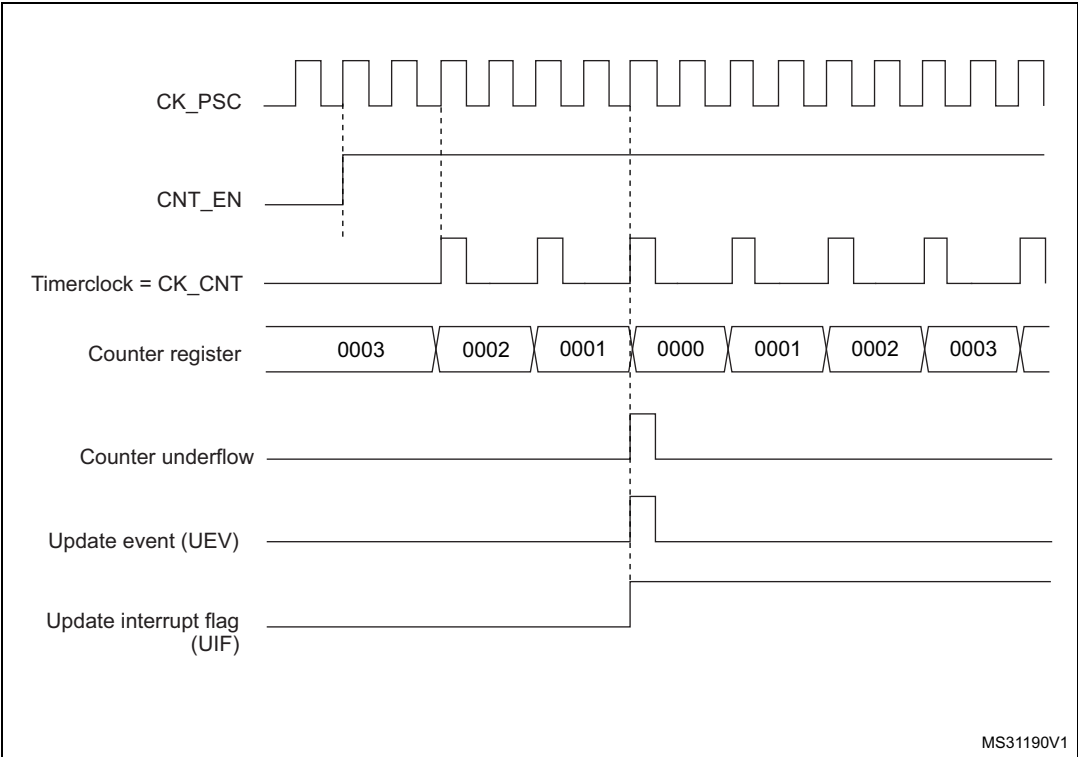
Figure 176. Counter timing diagram, internal clock divided by 2
