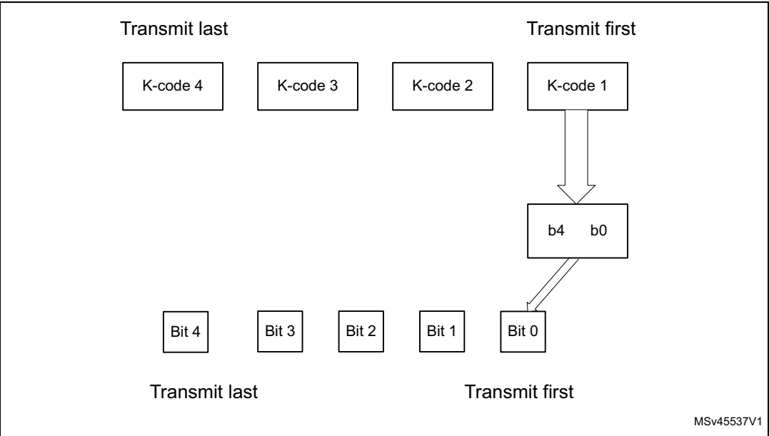
Figure 406. K-code transmission
