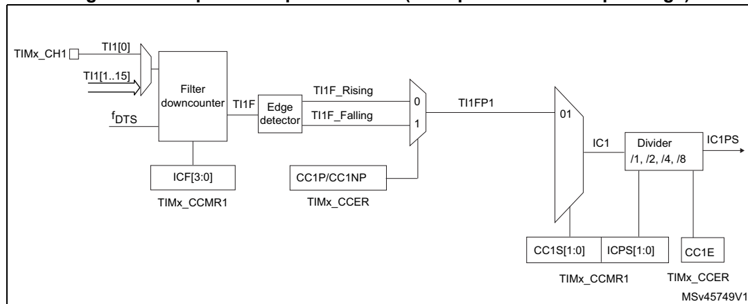
Figure 231. Capture/compare channel (example: channel 1 input stage)
