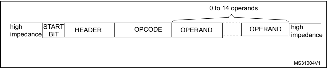
Figure 416. Message structure
