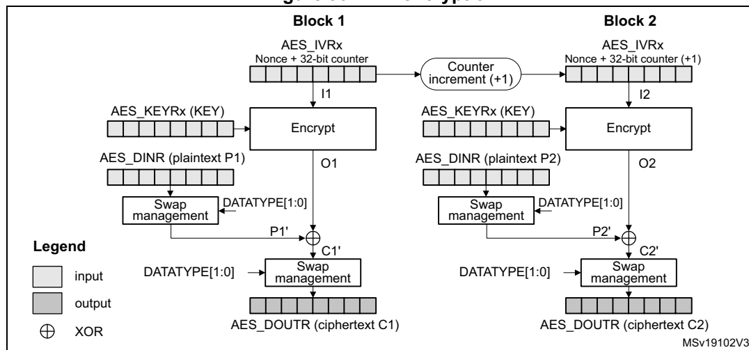
Figure 90. CTR encryption
