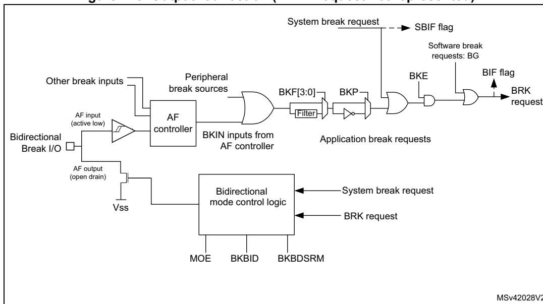
Figure 148. Output redirection (BRK2 request not represented)
