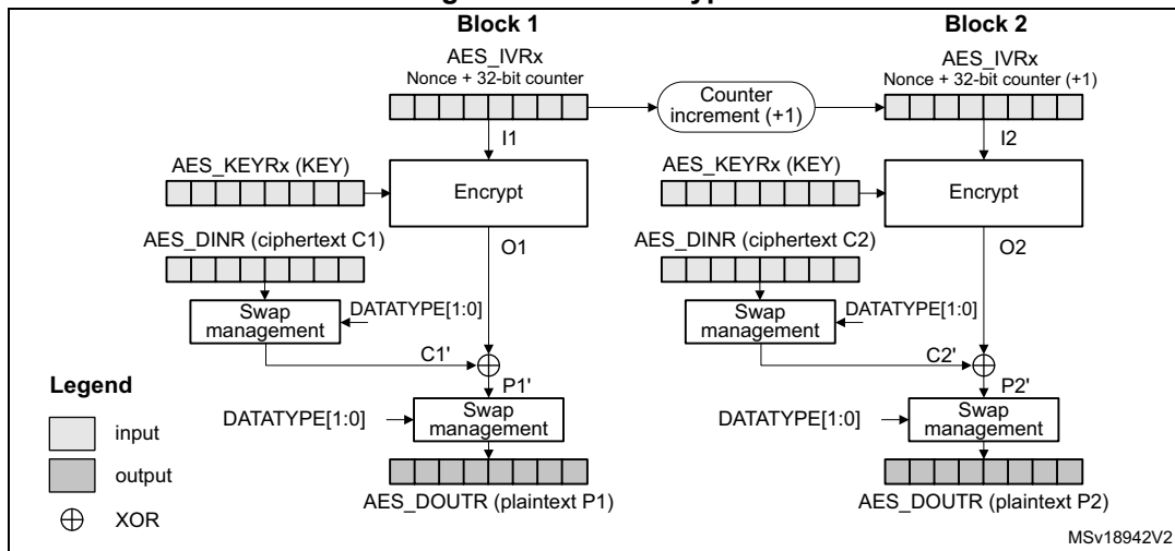
Figure 91. CTR decryption
