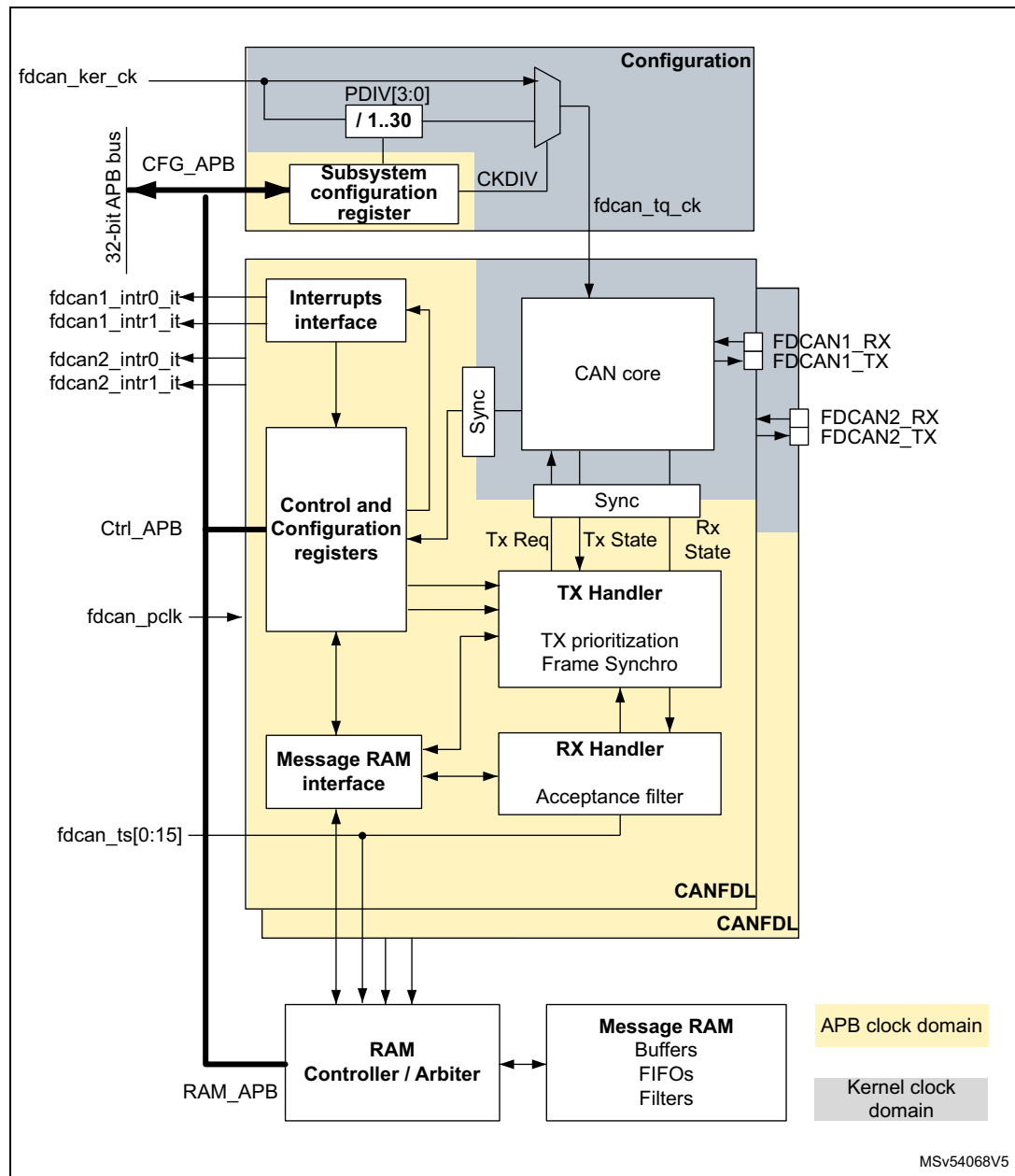
Figure 392. CAN subsystem.
