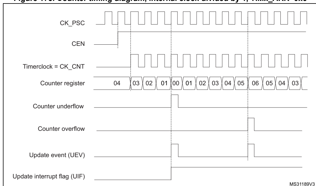
Figure 175. Counter timing diagram, internal clock divided by 1, TIMx_ARR=0x6
