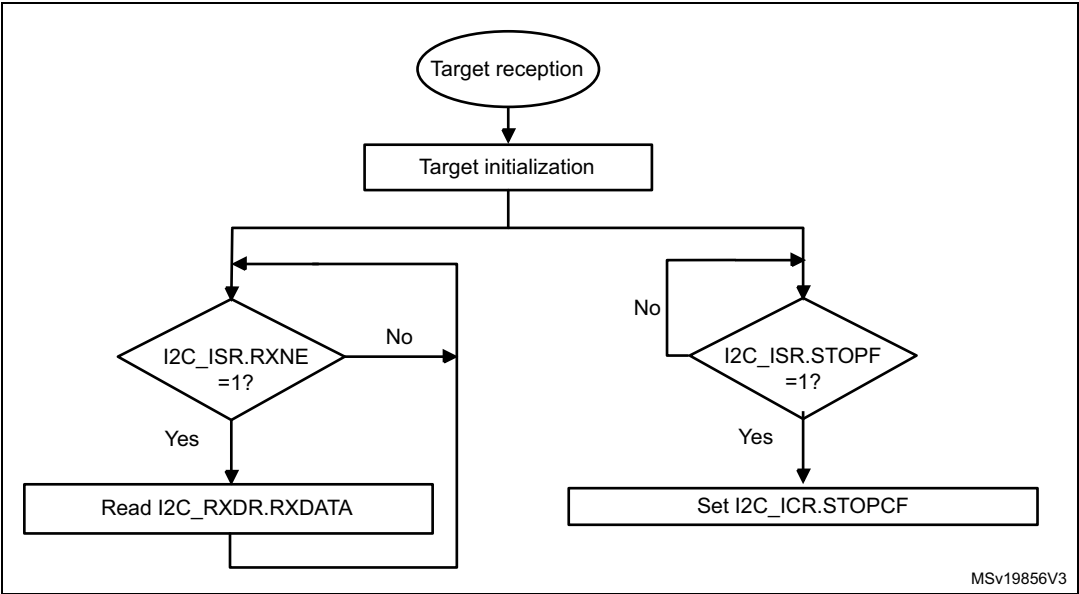
Figure 295. Transfer sequence flow for I2C target receiver, NOSTRETCH = 1
