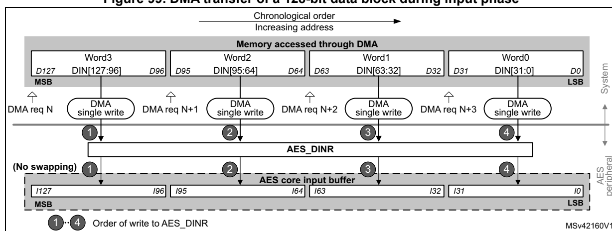
Figure 99. DMA transfer of a 128-bit data block during input phase
