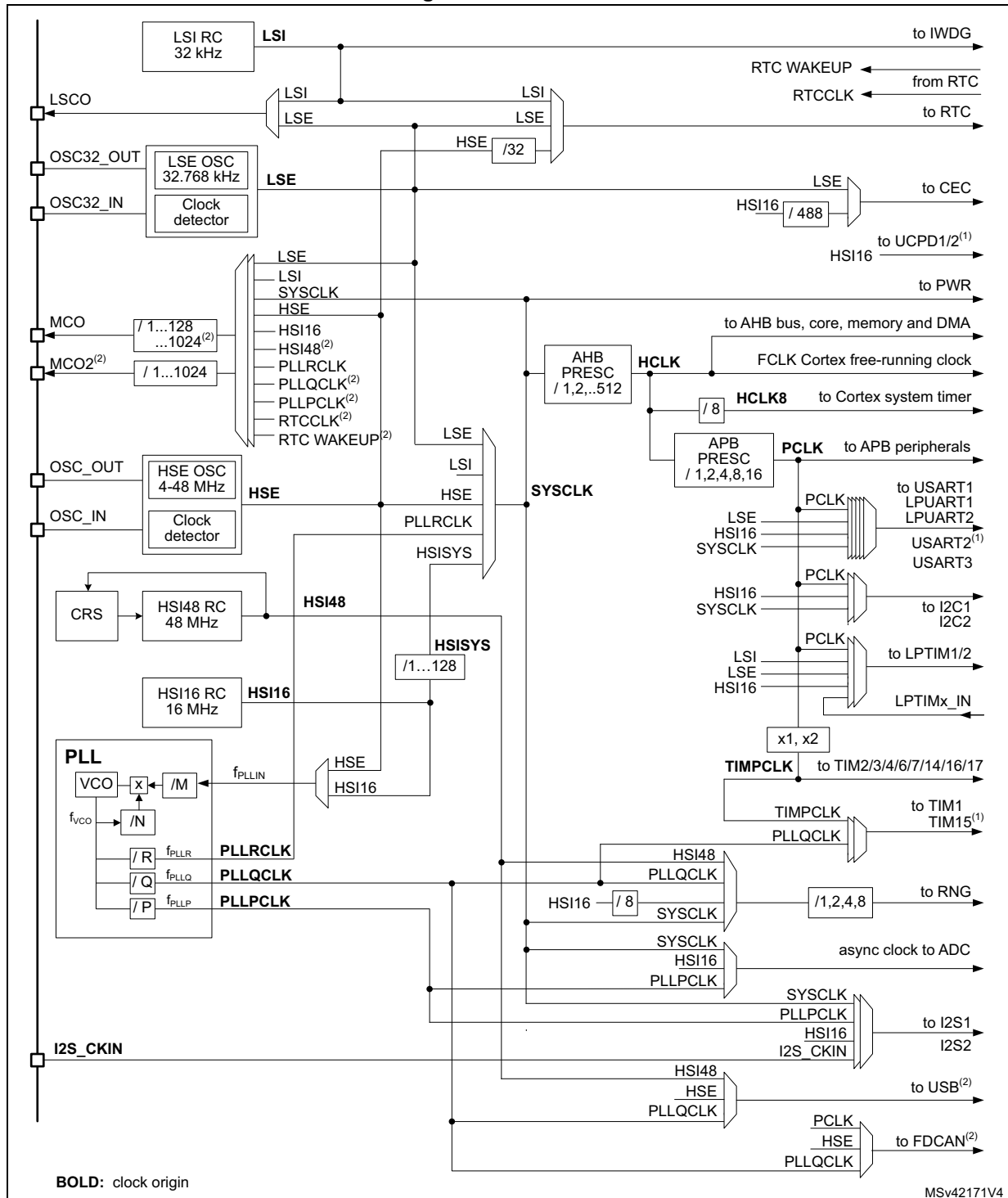
Figure 10. Clock tree
