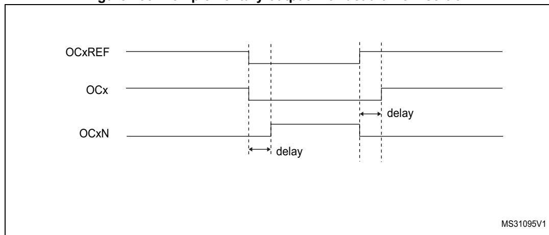
Figure 258. Complementary output with dead-time insertion.
