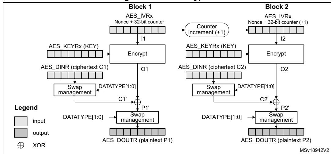
Figure 91. CTR decryption
