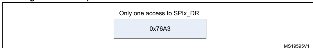
Figure 377. Example of 16-bit data frame extended to 32-bit channel frame
