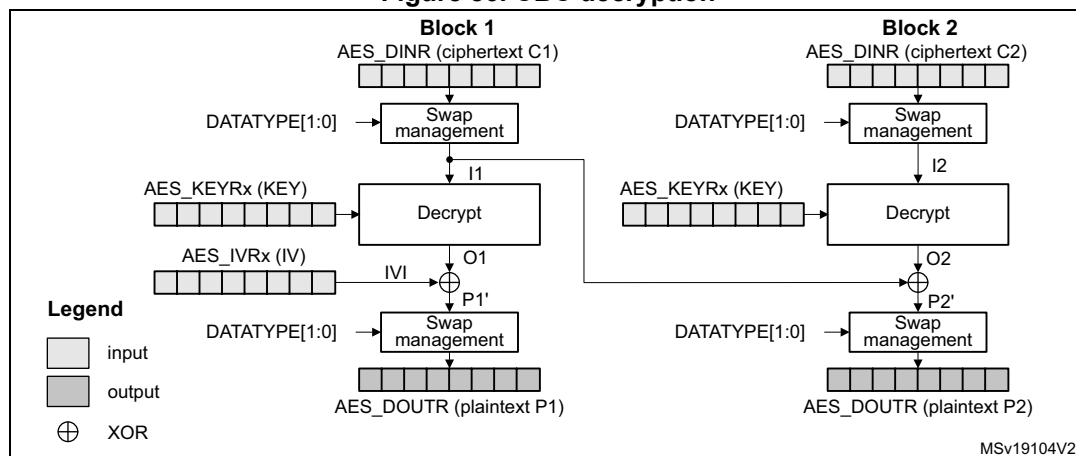
Figure 86. CBC decryption
