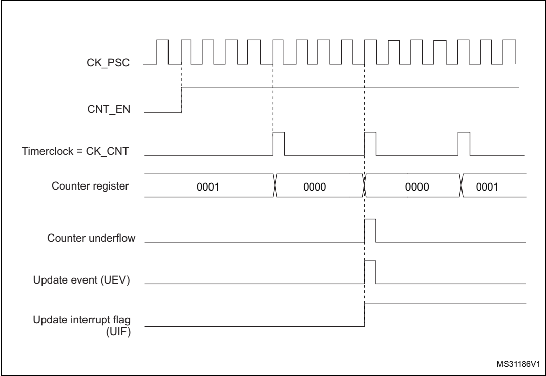
Figure 172. Counter timing diagram, internal clock divided by 4
