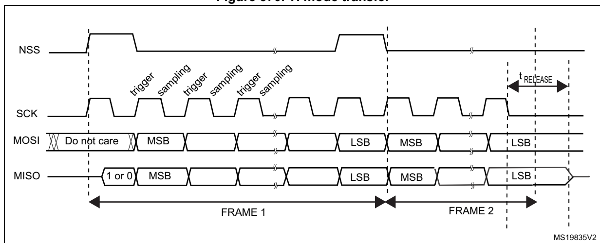
Figure 370. TI mode transfer
