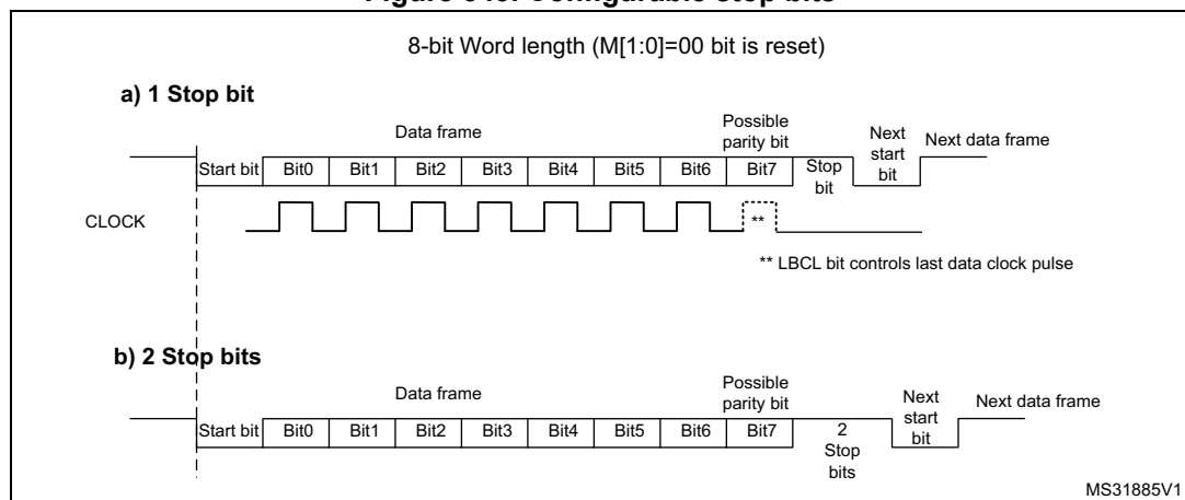
Figure 343. Configurable stop bits
