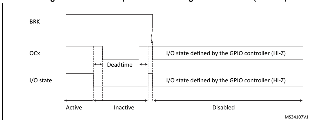
Figure 147. PWM output state following BRK assertion (OSSR=0)
