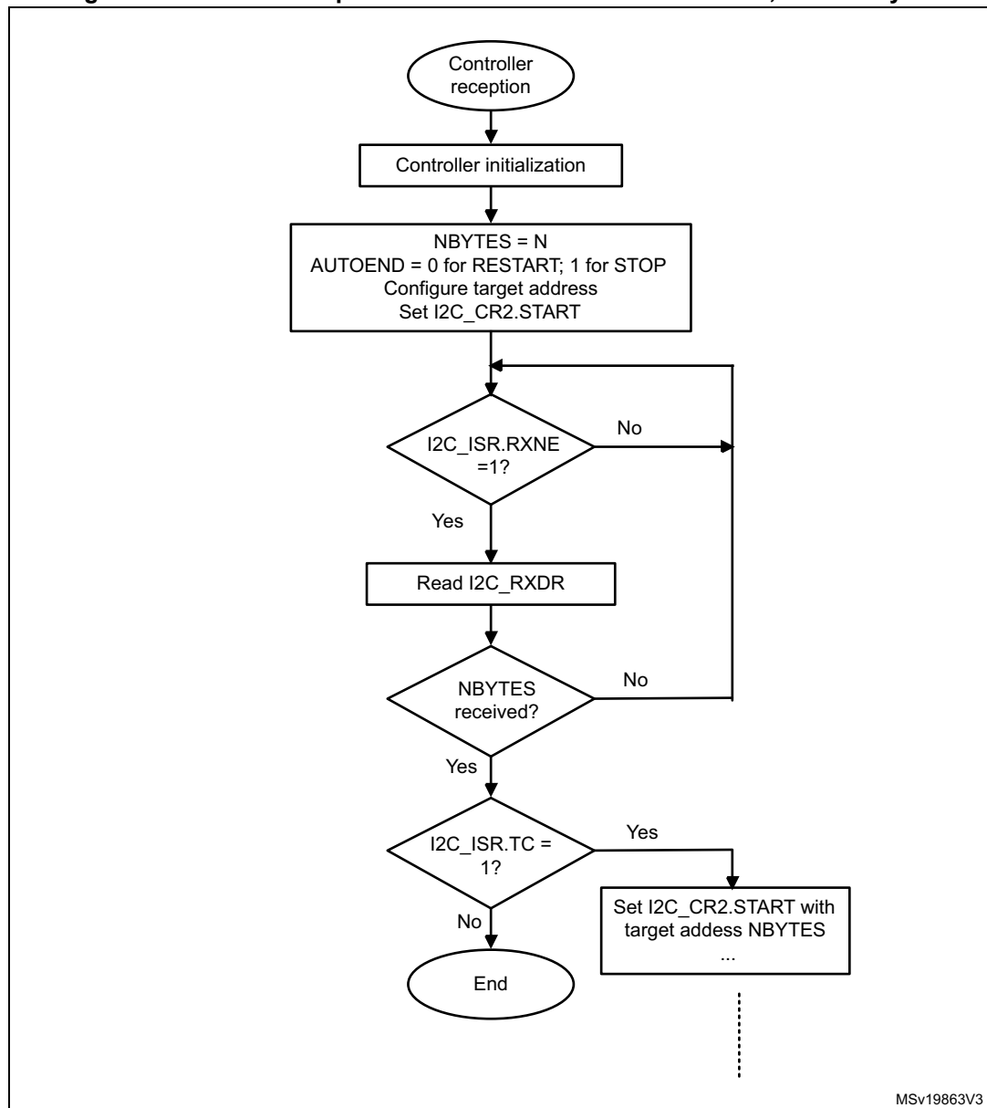
Figure 304. Transfer sequence flow for I2C controller receiver, N \leq 255 bytes
