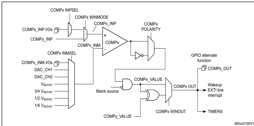
Figure 68. Comparator block diagram
