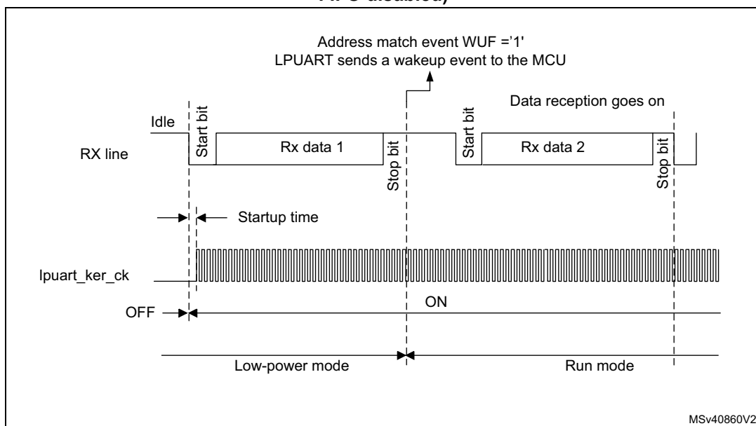
Figure 353. Wake-up event verified (wake-up event = address match, FIFO disabled)
