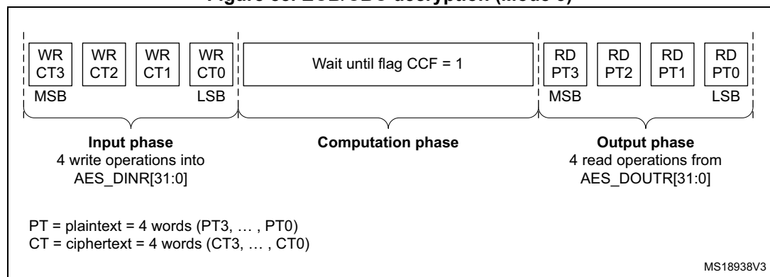
Figure 88. ECB/CBC decryption (Mode 3)
