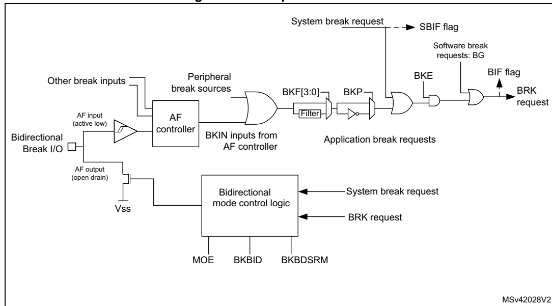
Figure 263. Output redirection
