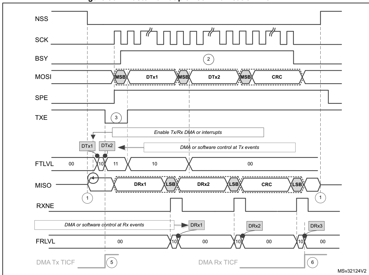
Figure 367. Master full-duplex communication with CRC
