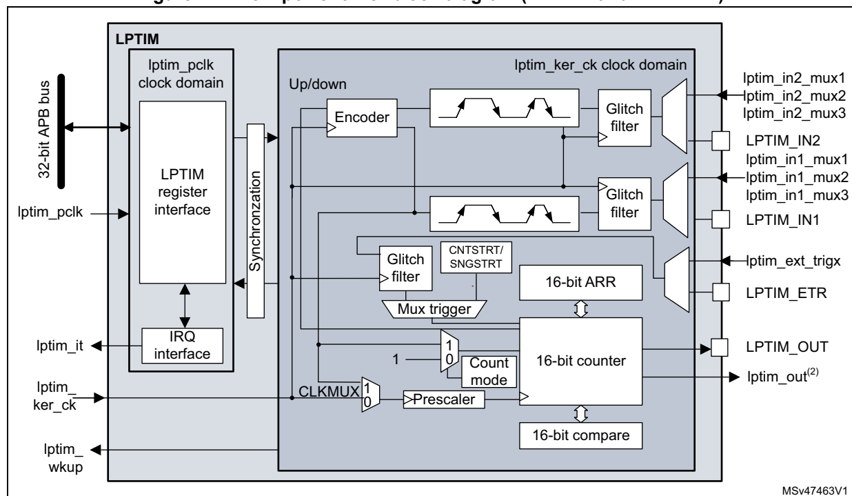
Figure 271. Low-power timer block diagram (LPTIM1 and LPTIM2 (1) )
