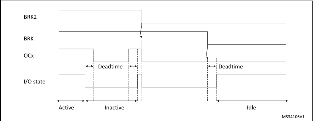
Figure 146. PWM output state following BRK and BRK2 pins assertion ( OSSl=1 )
