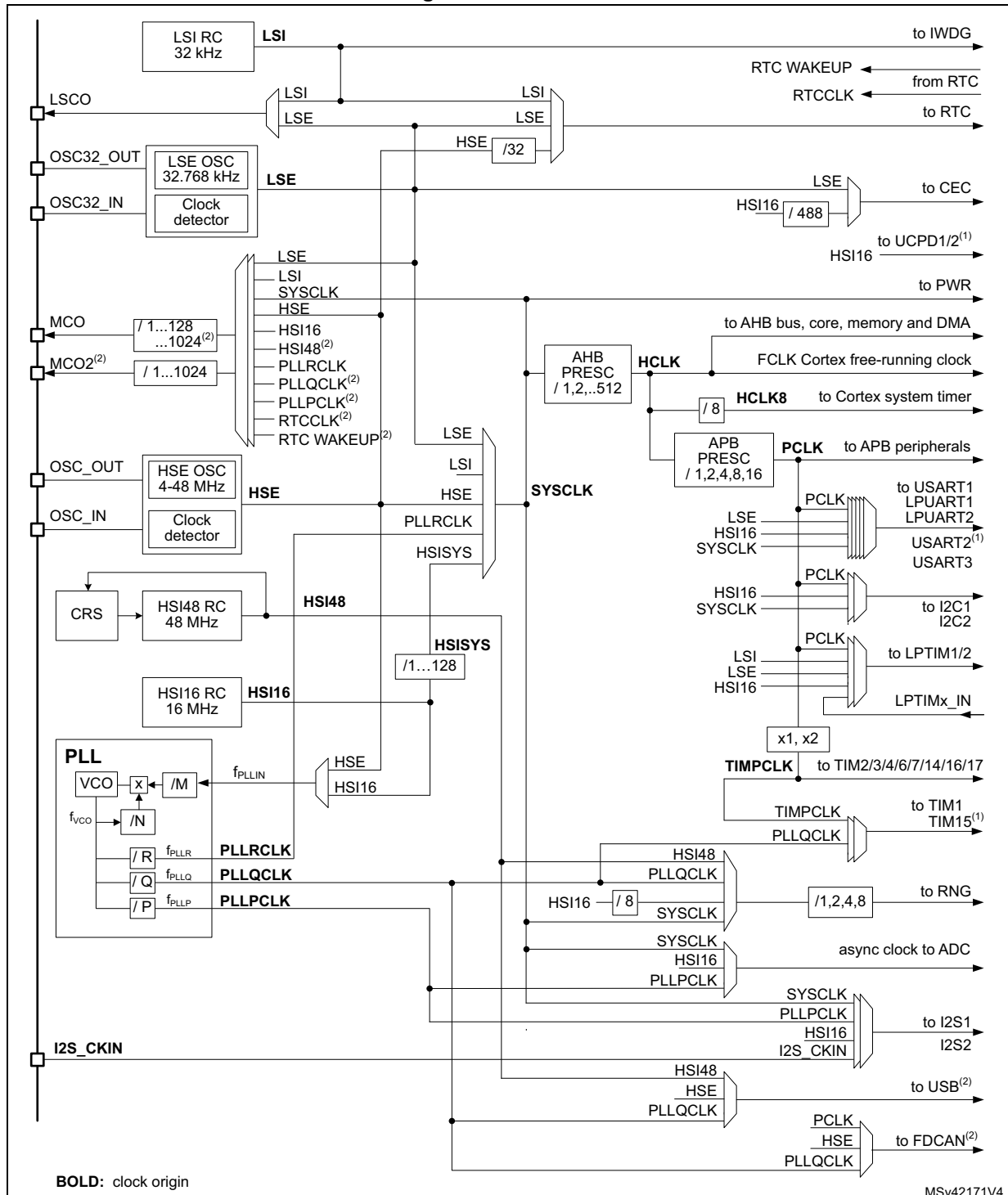
Figure 10. Clock tree
