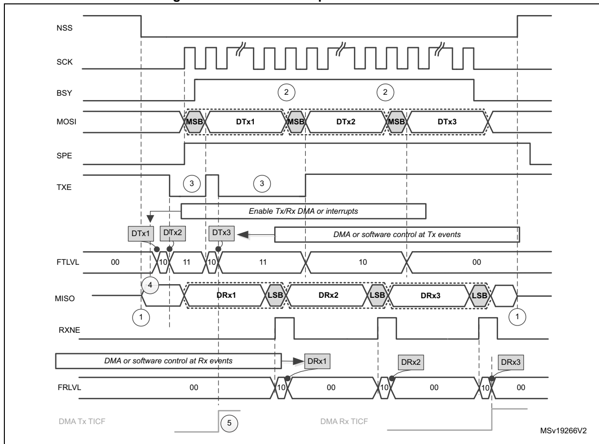
Figure 365. Master full-duplex communication
