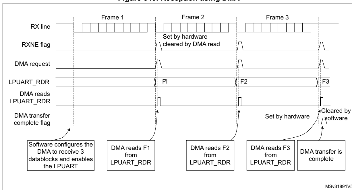
Figure 349. Reception using DMA
