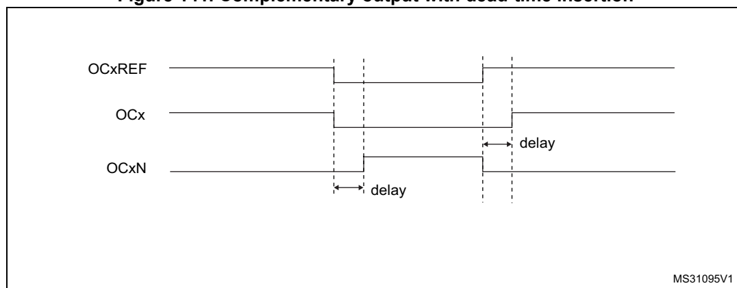
Figure 141. Complementary output with dead-time insertion
