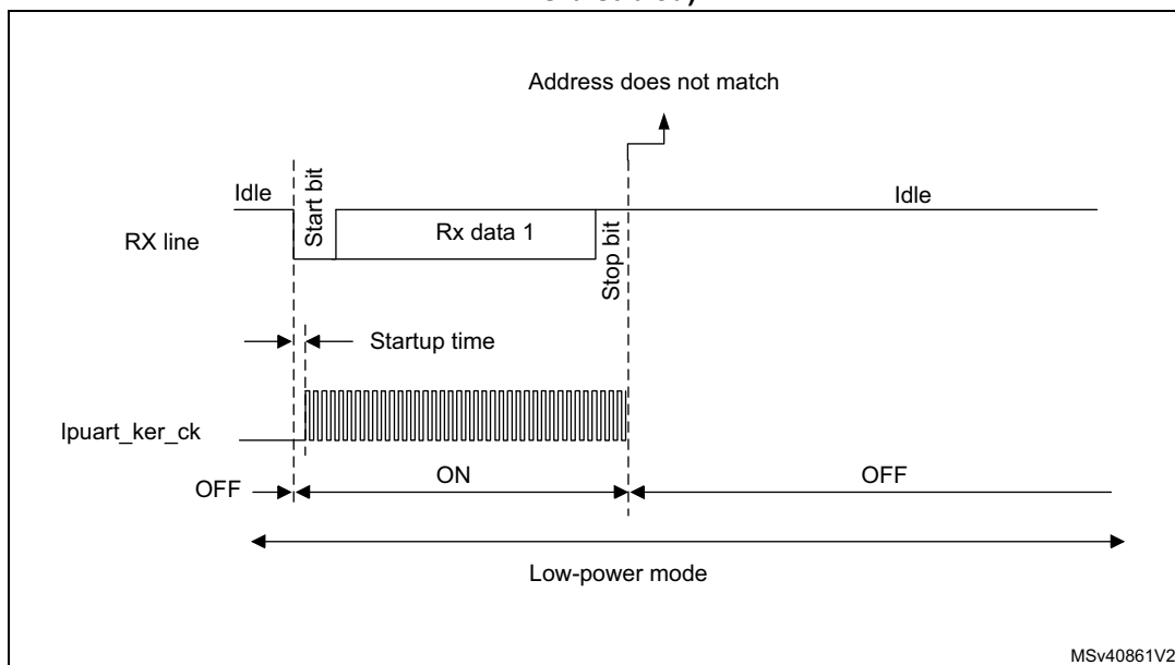
Figure 354. Wake-up event not verified (wake-up event = address match, FIFO disabled)
