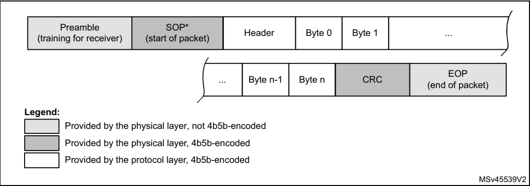
Figure 408. Packet format
