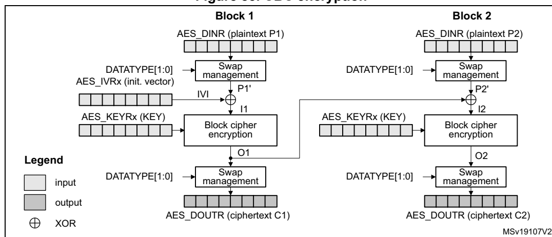
Figure 85. CBC encryption
