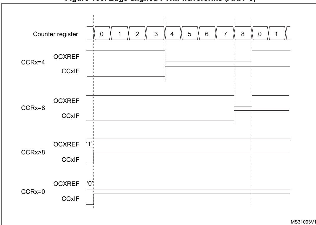
Figure 136. Edge-aligned PWM waveforms (ARR=8)
