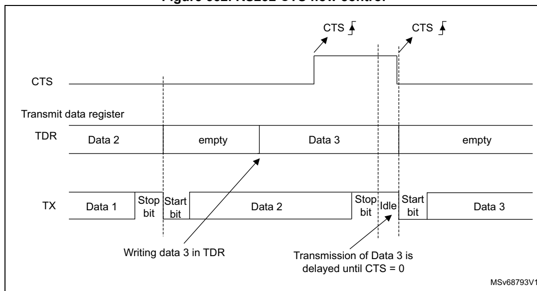
Figure 352. RS232 CTS flow control
