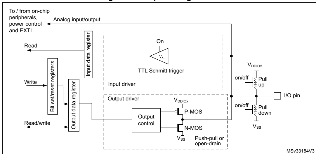
Figure 19. Output configuration
