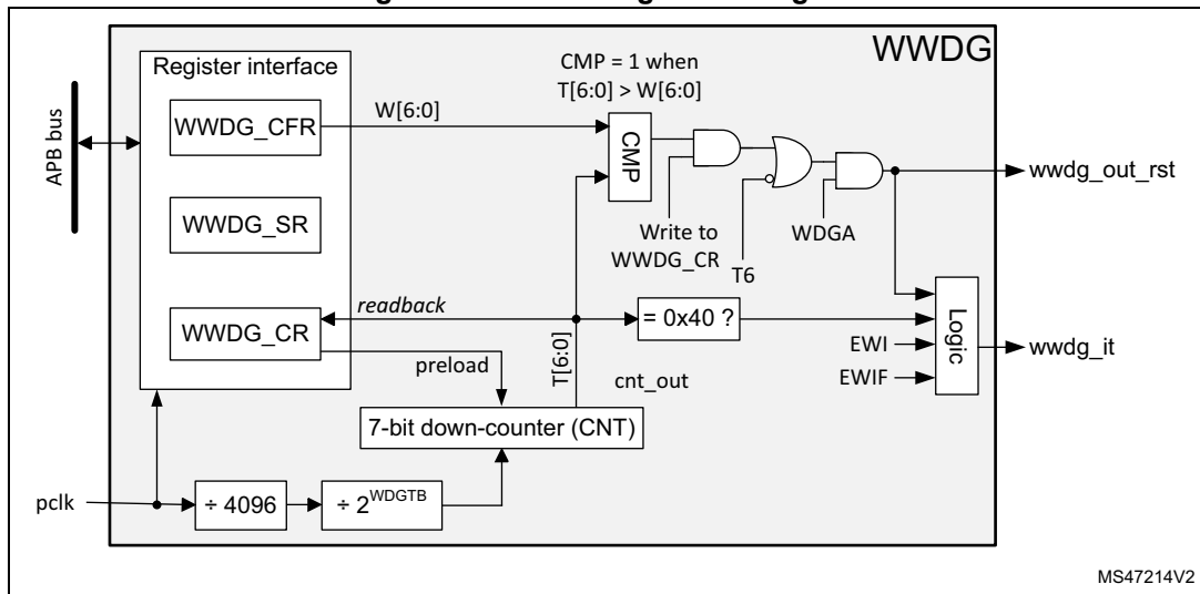
Figure 280. Watchdog block diagram
