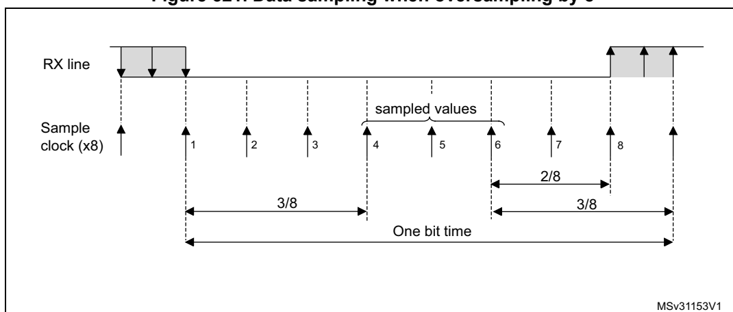
Figure 321. Data sampling when oversampling by 8
