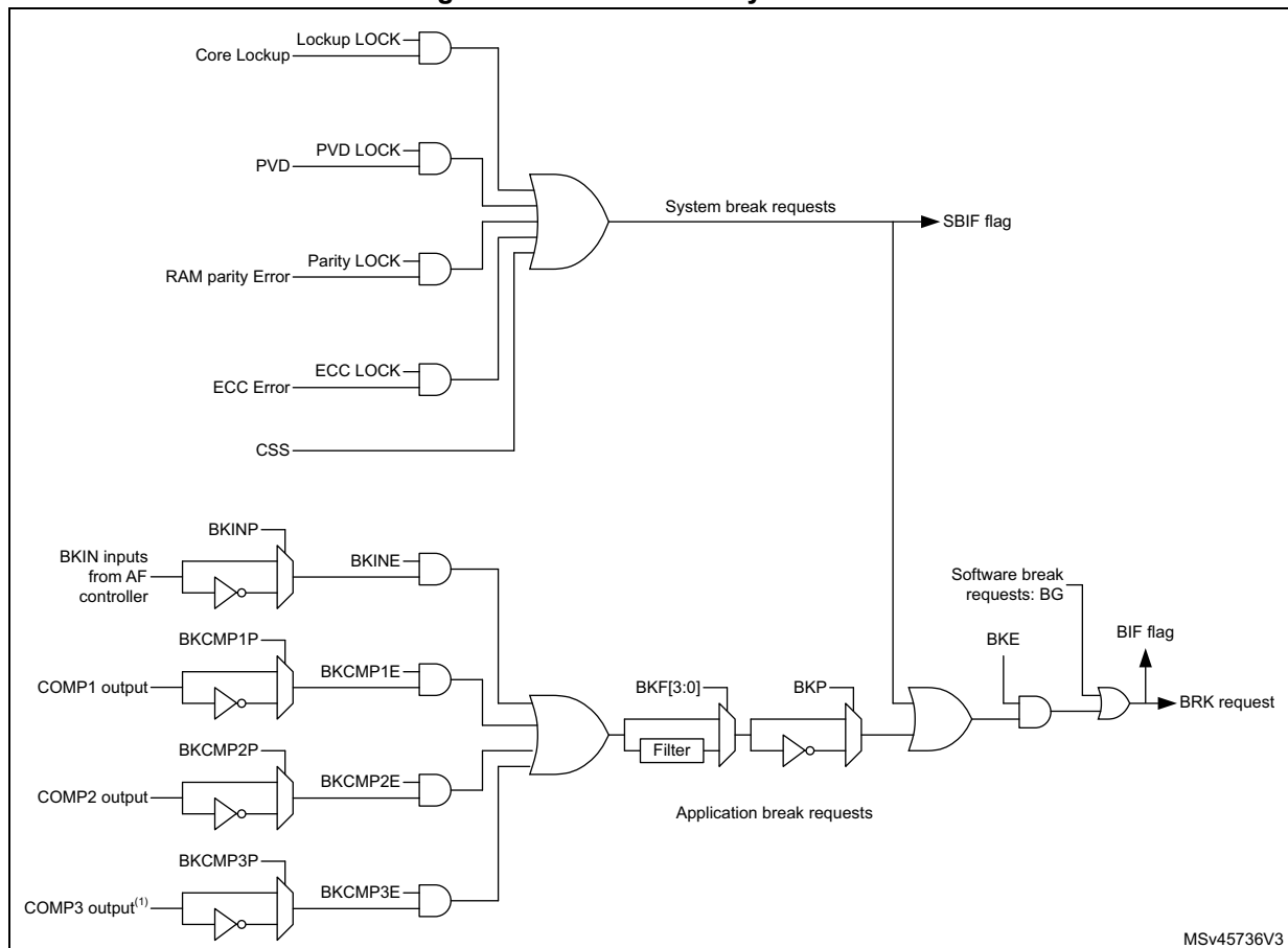
Figure 261. Break circuitry overview
