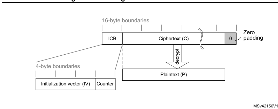
Figure 89. Message construction in CTR mode
