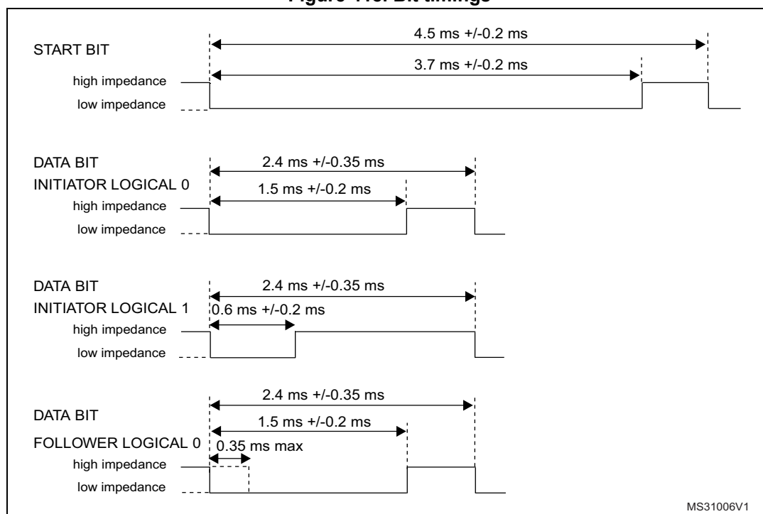
Figure 418. Bit timings
