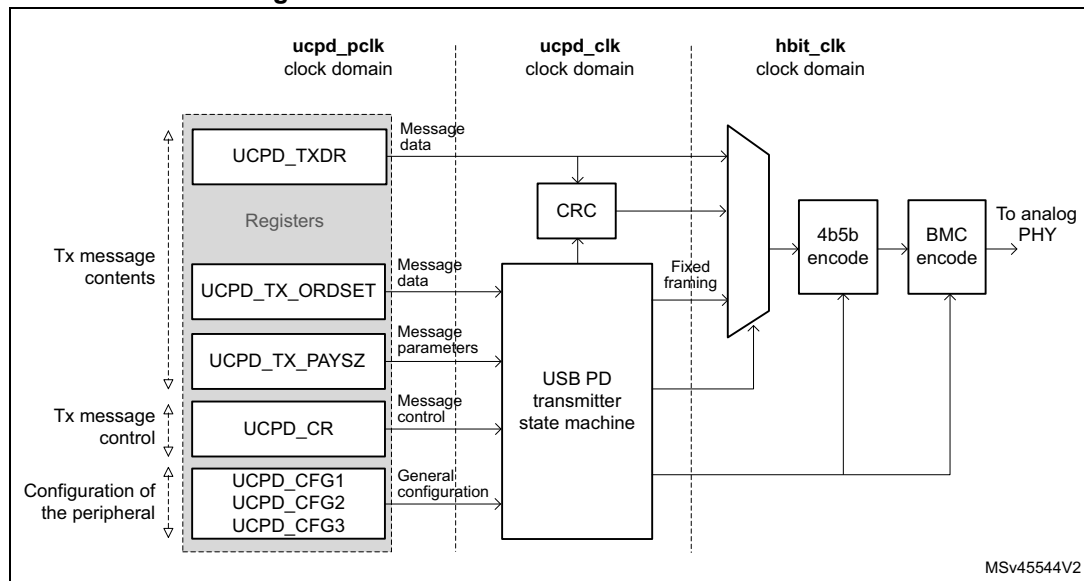
Figure 413. UCPD BMC transmitter architecture
