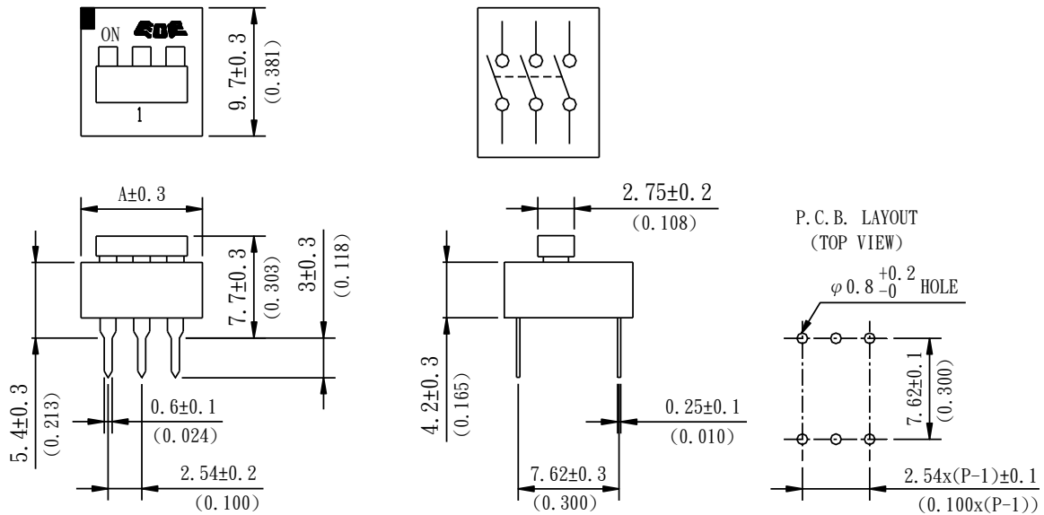
Dimension A
