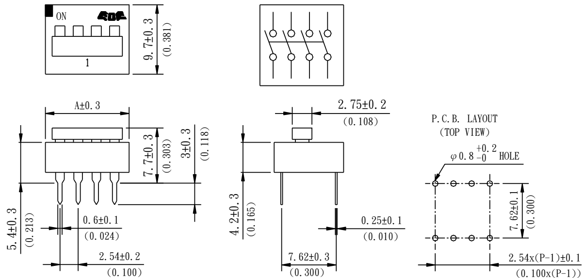
Dimension A
