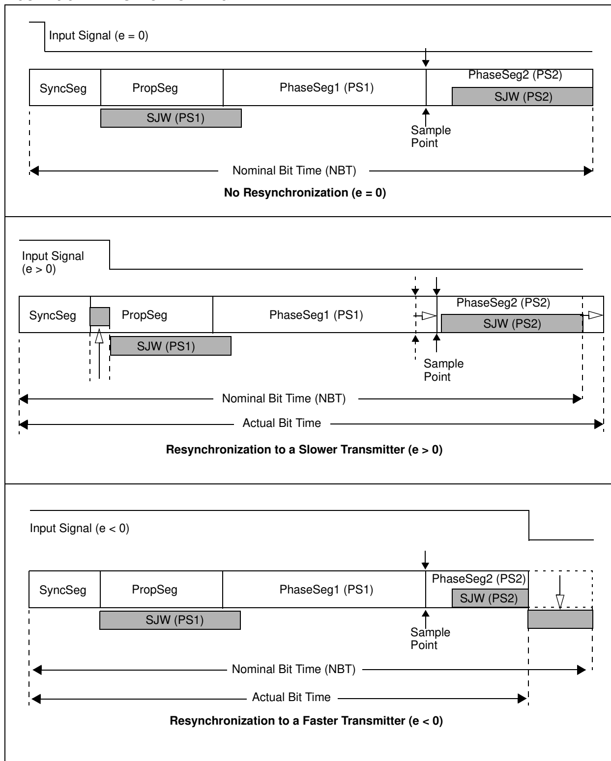
FIGURE 5-3: SYNCHRONIZING THE BIT TIME
