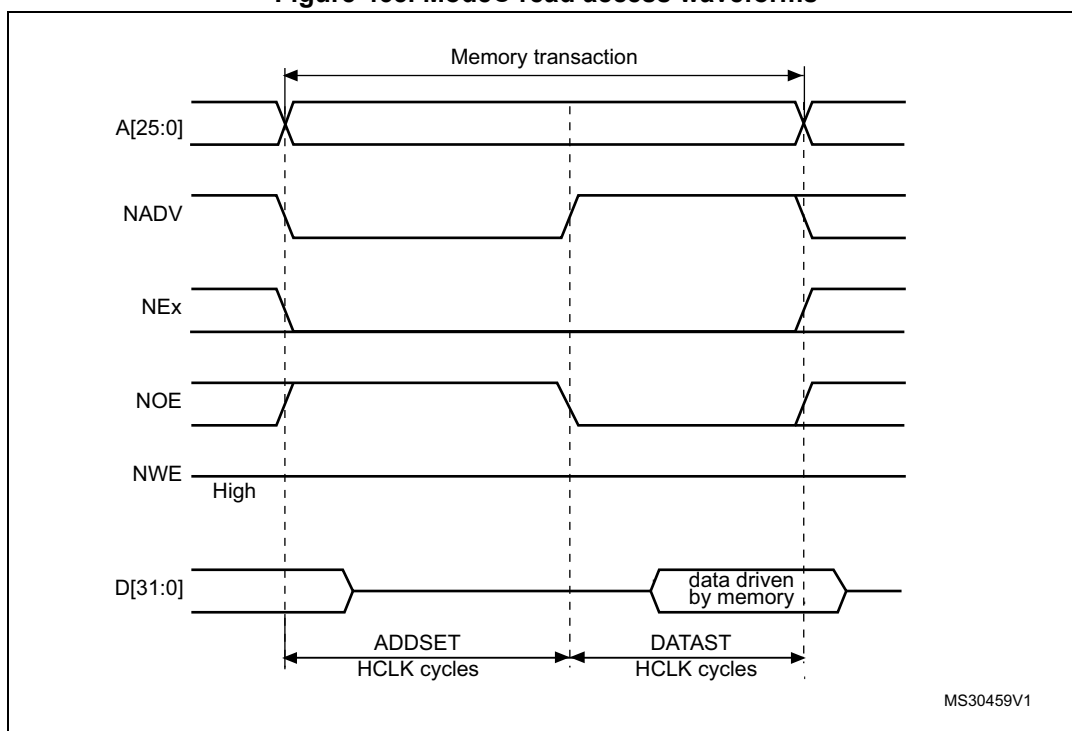
Figure 465. ModeC read access waveforms
