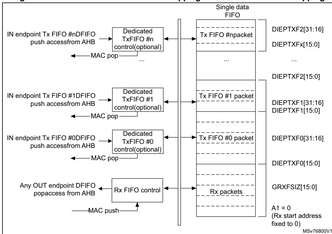
Figure 392. Device-mode FIFO address mapping and AHB FIFO access mapping
