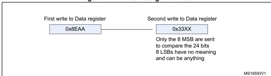
Figure 266. Transmitting 0x8EAA33
