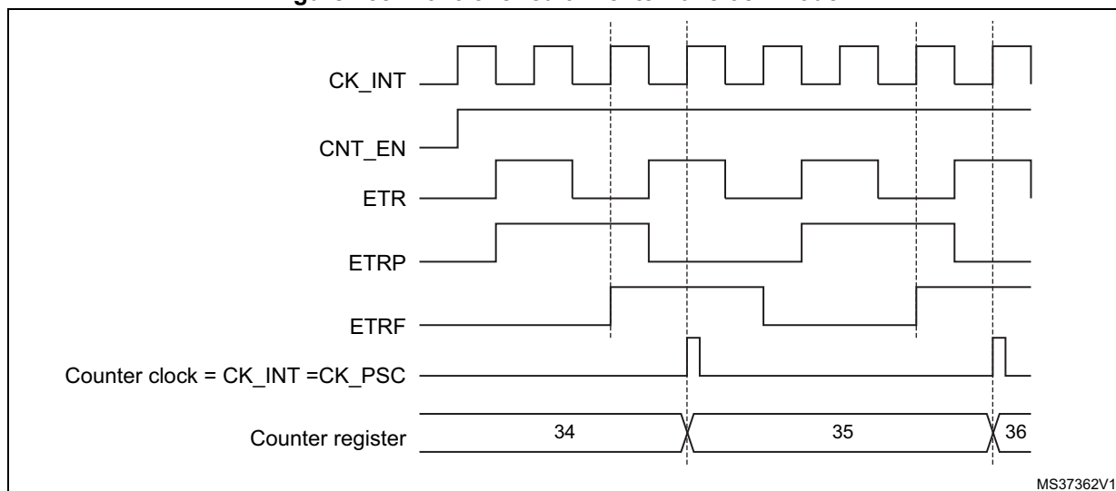
Figure 158. Control circuit in external clock mode 2
