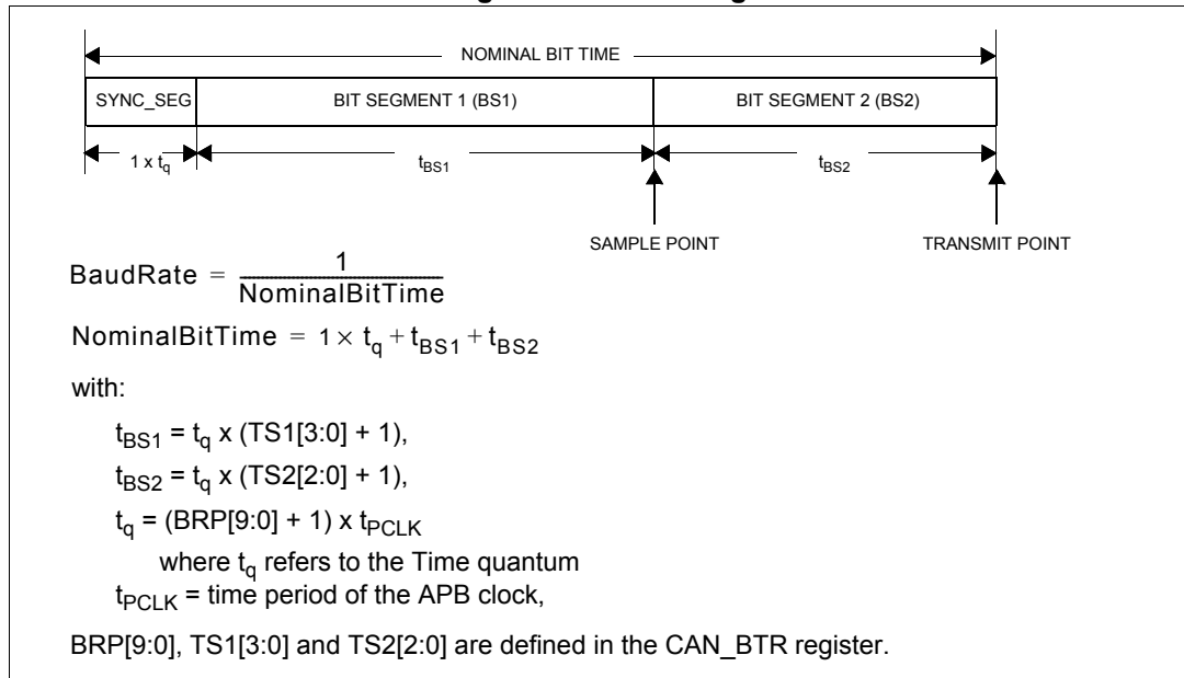
Figure 346. Bit timing
