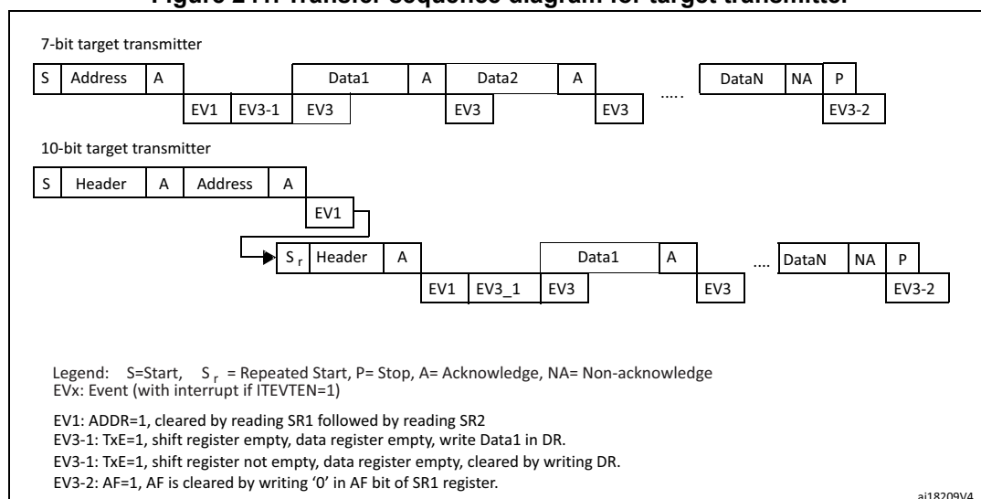
Figure 241. Transfer sequence diagram for target transmitter
