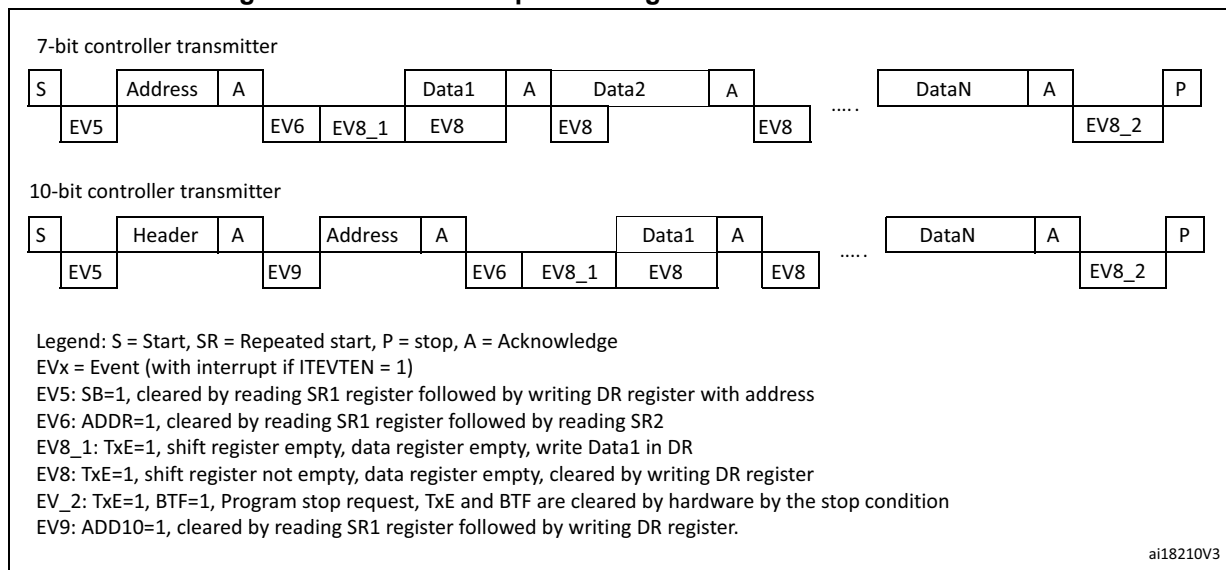
Figure 243. Transfer sequence diagram for controller transmitter
