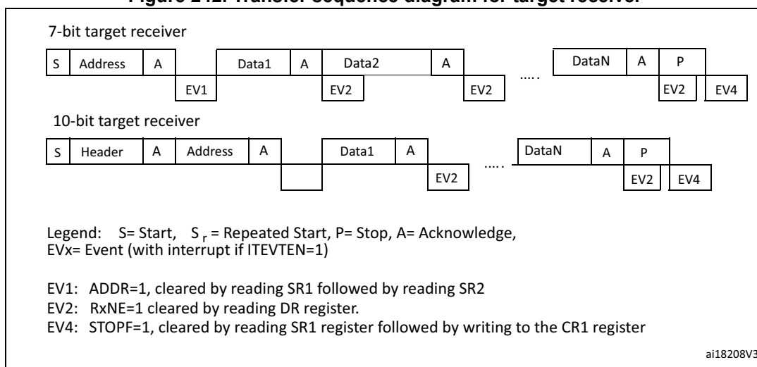
Figure 242. Transfer sequence diagram for target receiver
