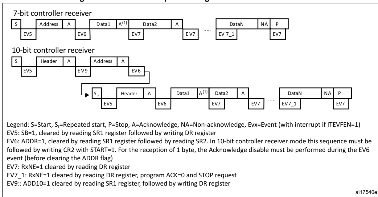
Figure 244. Transfer sequence diagram for controller receiver
