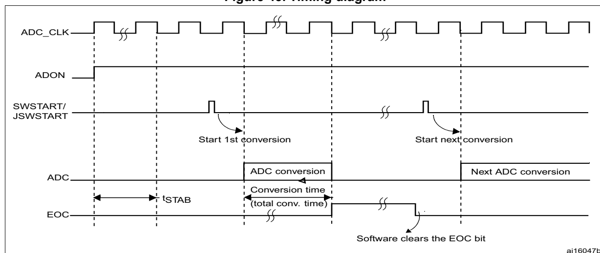
Figure 45. Timing diagram
