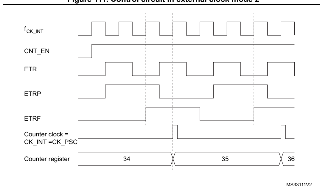
Figure 111. Control circuit in external clock mode 2
