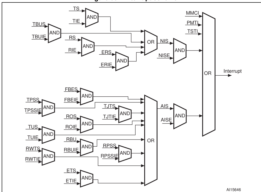
Figure 384. Interrupt scheme
