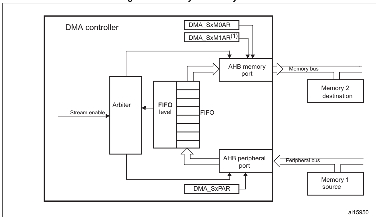
Figure 38. Memory-to-memory mode
