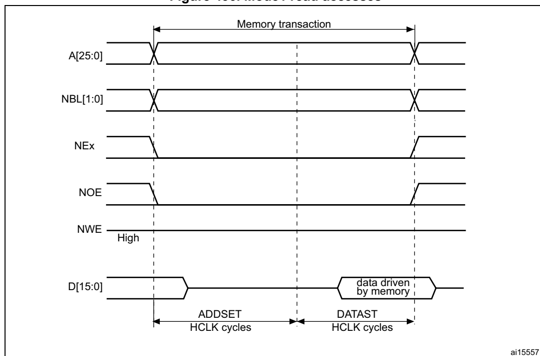
Figure 436. Mode1 read accesses
