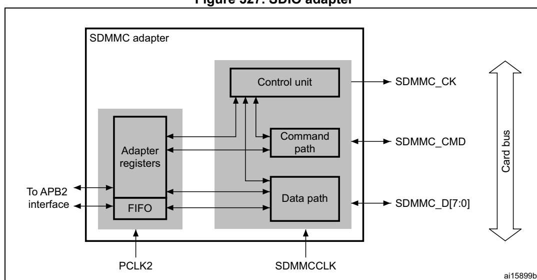
Figure 327. SDIO adapter
